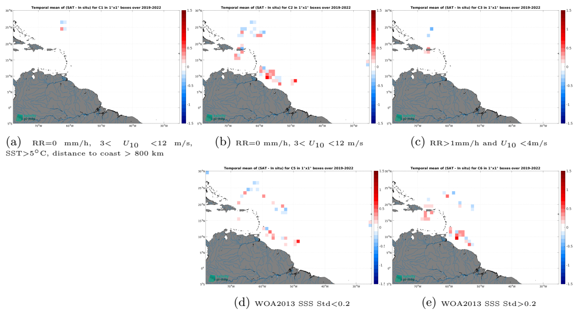
Figure 14: Temporal mean gridded over spatial boxes of size 1^\circ \times 1^\circ of \Delta SSS (CCI SSS L4 Merged-OI v5.5 - 7-day running (ESA) - Sailydrone) for 5 different subdatasets corresponding to:RR=0 mm/h, 3 < U_{10} < 12 m/s, SST >5^\circ C, distance to coast > 800 km (a), RR=0 mm/h, 3 < U_{10} < 12 m/s (b), RR >1 mm/h and U_{10} < 4 m/s (c), WOA2013 SSS Std <0.2 (d), WOA2013 SSS Std >0.2 (e).
