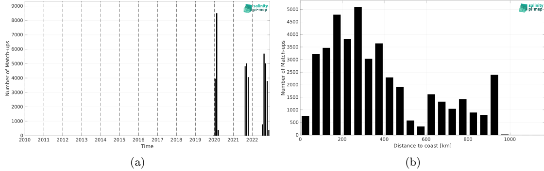
Figure 2: Number of match-ups between Saildrone and CCI SSS L4 Merged-OI v5.5 - 7-day running (ESA) SSS as a function of time (a) and as function of the distance to coast (b) over the Amazon and Orinoco river plumes Pi-MEP region and for the full satellite product period.
