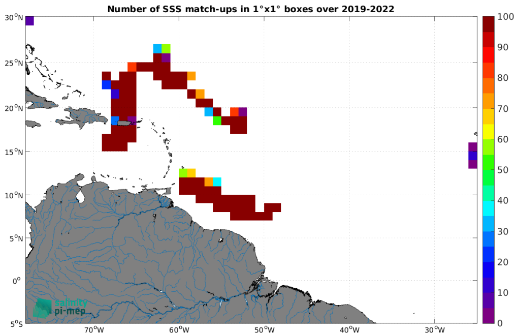
Figure 5: Number of SSS match-ups between Saildrone SSS and the CCI SSS L4 Merged-OI v5.5 - 7-day running (ESA) SSS product for the Amazon and Orinoco river plumes Pi-MEP region over 1^\circ \times 1^\circ boxes and for the full satellite product period.
