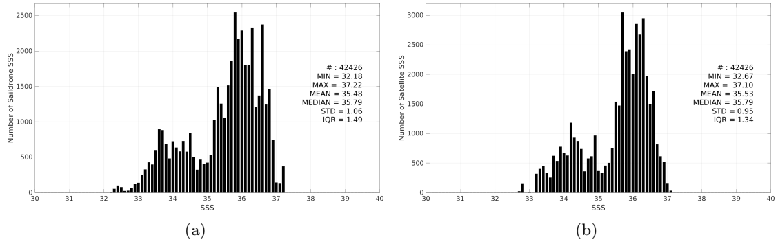
Figure 3: Histograms of SSS from Saildrone (a) and CCI SSS L4 Merged-OI v5.5 - 7-day running (ESA) (b) considering all match-up pairs per bins of 0.1 over the Amazon and Orinoco river plumes Pi-MEP region and for the full satellite product period.
