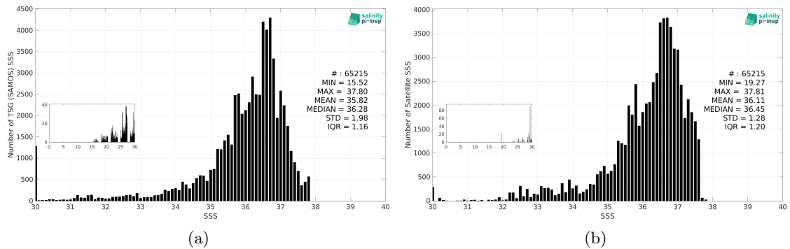
Figure 3: Histograms of SSS from TSG (SAMOS) (a) and CCI SSS L4 Merged-OI v5.5 - 30-day running (ESA) (b) considering all match-up pairs per bins of 0.1 over the Amazon and Orinoco river plumes Pi-MEP region and for the full satellite product period.
