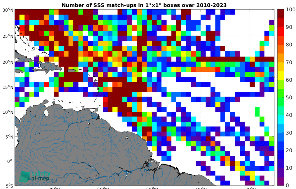
Figure 5: Number of SSS match-ups between TSG (SAMOS) SSS and the CCI SSS L4 Merged-OI v5.5 - 30-day running (ESA) SSS product for the Amazon and Orinoco river plumes Pi-MEP region over 1^\circ \times 1^\circ boxes and for the full satellite product period.
