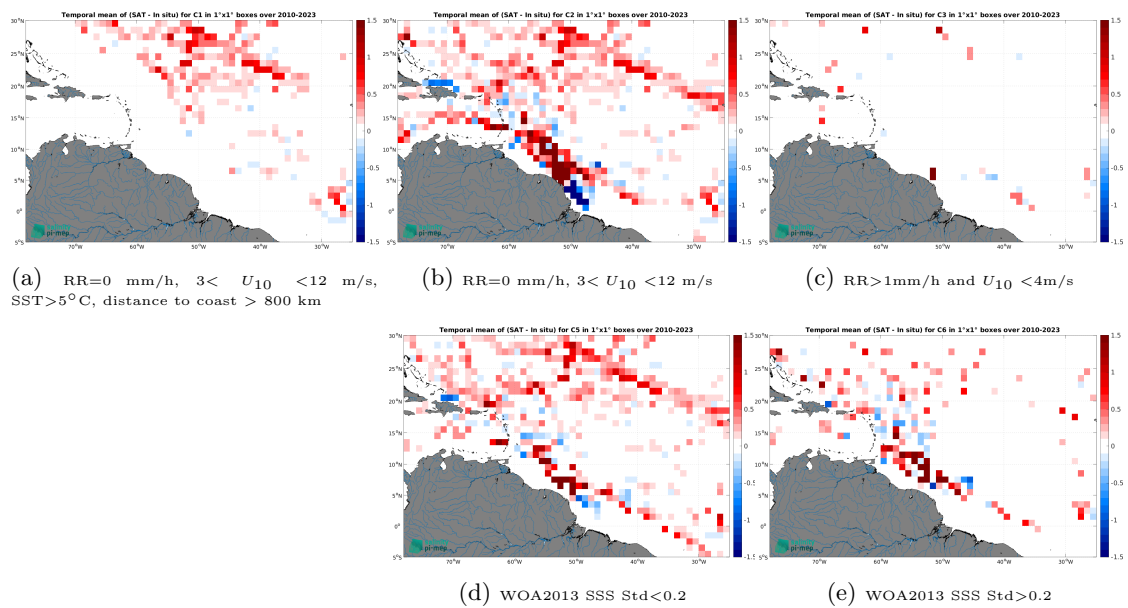
Figure 14: Temporal mean gridded over spatial boxes of size 1^\circ \times 1^\circ of \Delta\text{SSS} (CCI SSS L4 Merged-OI v5.5 - 30-day running (ESA) - TSG (SAMOS)) for 5 different subdatasets corresponding to:RR=0 mm/h, 3 < U_{10} < 12 m/s, SST >5^\circ\text{C} , distance to coast > 800 km (a), RR=0 mm/h, 3 < U_{10} < 12 m/s (b), RR >1 mm/h and U_{10} < 4 m/s (c), WOA2013 SSS Std <0.2 (d), WOA2013 SSS Std >0.2 (e).
