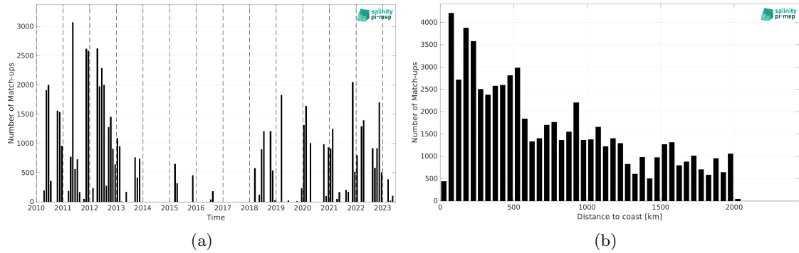
Figure 2: Number of match-ups between TSG (SAMOS) and CCI SSS L4 Merged-OI v5.5 - 30-day running (ESA) SSS as a function of time (a) and as function of the distance to coast (b) over the Amazon and Orinoco river plumes Pi-MEP region and for the full satellite product period.
