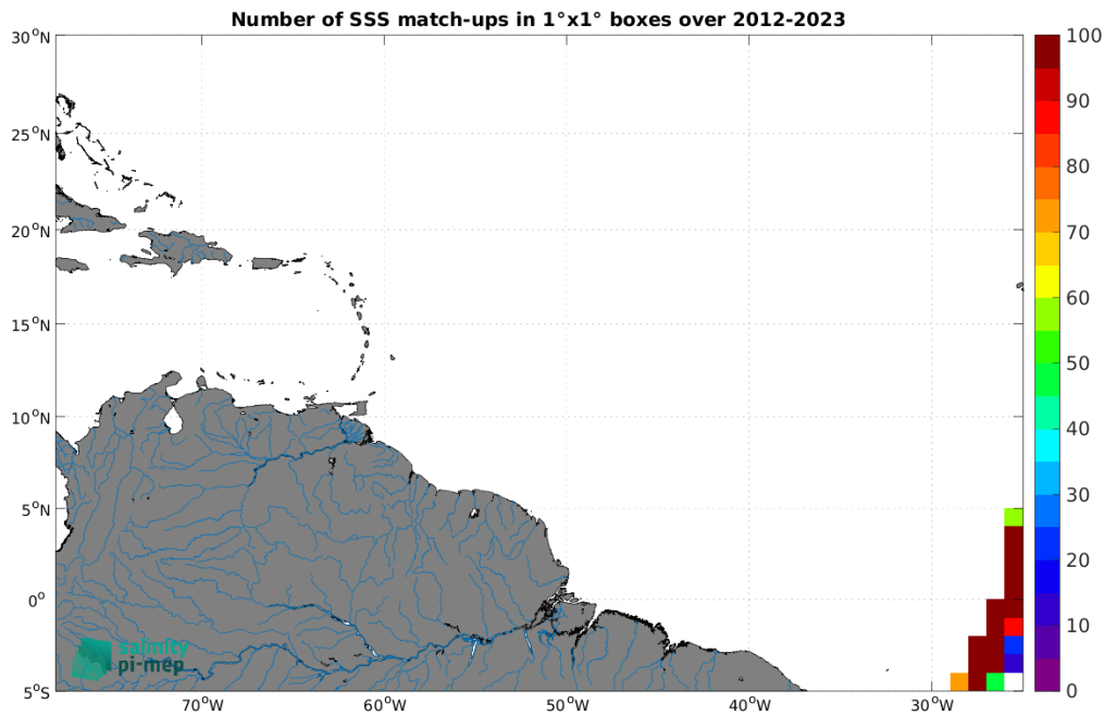
Figure 5: Number of SSS match-ups between TSG (Polarstern) SSS and the CCI SSS L4 Merged-OI v5.5 - 30-day running (ESA) SSS product for the Amazon and Orinoco river plumes Pi-MEP region over 1^\circ \times 1^\circ boxes and for the full satellite product period.
