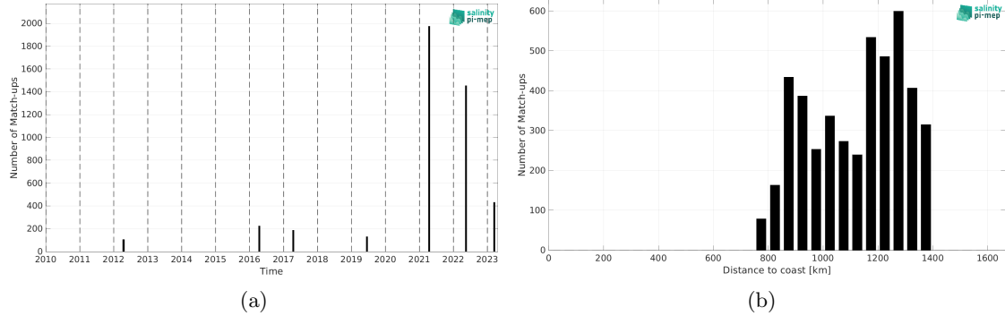
Figure 2: Number of match-ups between TSG (Polarstern) and CCI SSS L4 Merged-OI v5.5 - 30-day running (ESA) SSS as a function of time (a) and as function of the distance to coast (b) over the Amazon and Orinoco river plumes Pi-MEP region and for the full satellite product period.
