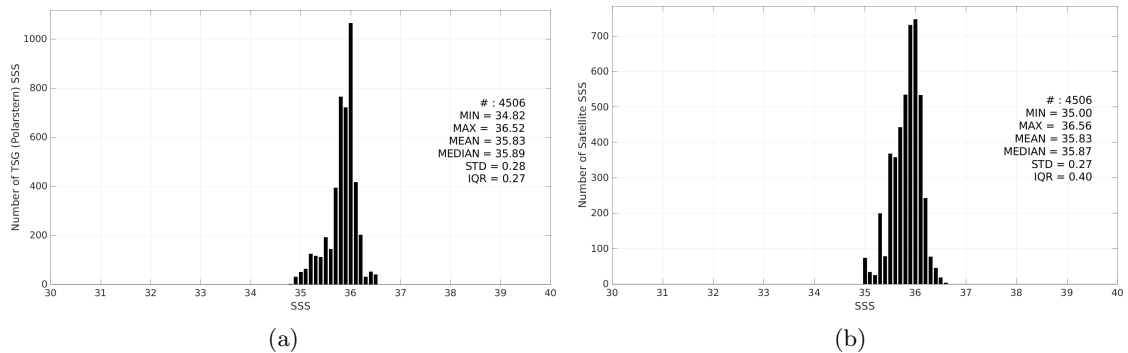
Figure 3: Histograms of SSS from TSG (Polarstern) (a) and CCI SSS L4 Merged-OI v5.5 - 30-day running (ESA) (b) considering all match-up pairs per bins of 0.1 over the Amazon and Orinoco river plumes Pi-MEP region and for the full satellite product period.
