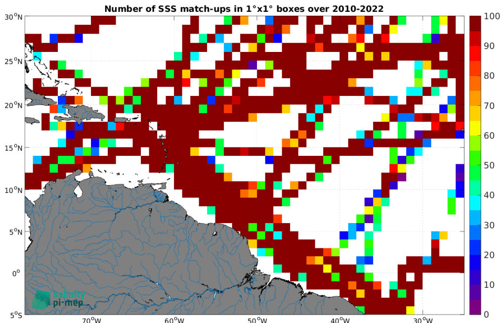
Figure 5: Number of SSS match-ups between TSG (GOSUD-Research-vessel) SSS and the CCI SSS L4 Merged-OI v5.5 - 30-day running (ESA) SSS product for the Amazon and Orinoco river plumes Pi-MEP region over 1^\circ \times 1^\circ boxes and for the full satellite product period.
