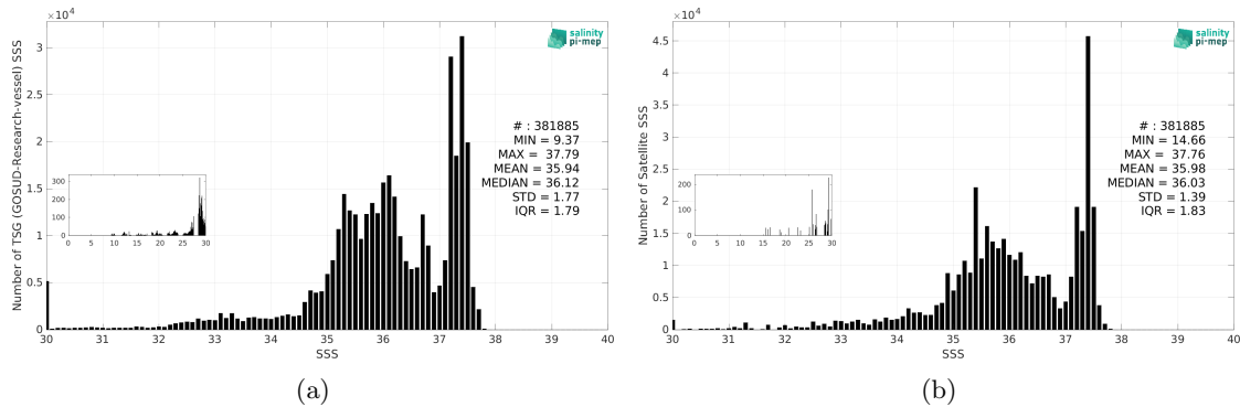
Figure 3: Histograms of SSS from TSG (GOSUD-Research-vessel) (a) and CCI SSS L4 Merged-OI v5.5 - 30-day running (ESA) (b) considering all match-up pairs per bins of 0.1 over the Amazon and Orinoco river plumes Pi-MEP region and for the full satellite product period.
