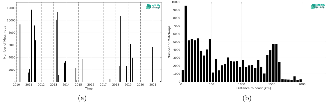
Figure 2: Number of match-ups between TSG (CSIC-UTM) and CCI SSS L4 Merged-OI v5.5 - 30-day running (ESA) SSS as a function of time (a) and as function of the distance to coast (b) over the Amazon and Orinoco river plumes Pi-MEP region and for the full satellite product period.
