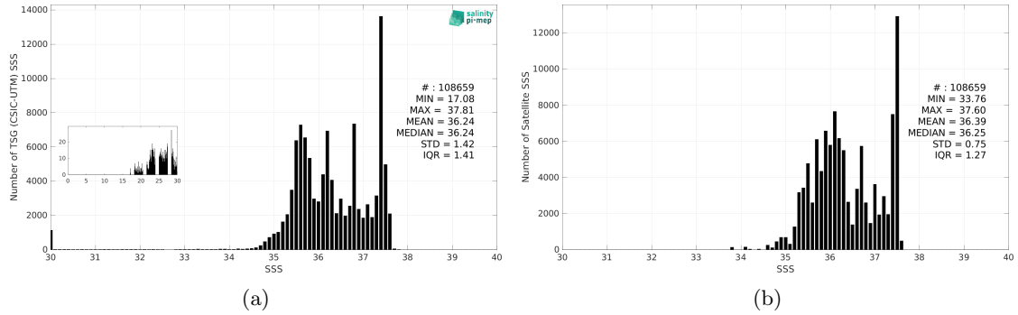
Figure 3: Histograms of SSS from TSG (CSIC-UTM) (a) and CCI SSS L4 Merged-OI v5.5 - 30-day running (ESA) (b) considering all match-up pairs per bins of 0.1 over the Amazon and Orinoco river plumes Pi-MEP region and for the full satellite product period.
