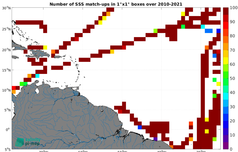
Figure 5: Number of SSS match-ups between TSG (CSIC-UTM) SSS and the CCI SSS L4 Merged-OI v5.5 - 30-day running (ESA) SSS product for the Amazon and Orinoco river plumes Pi-MEP region over 1^\circ \times 1^\circ boxes and for the full satellite product period.
