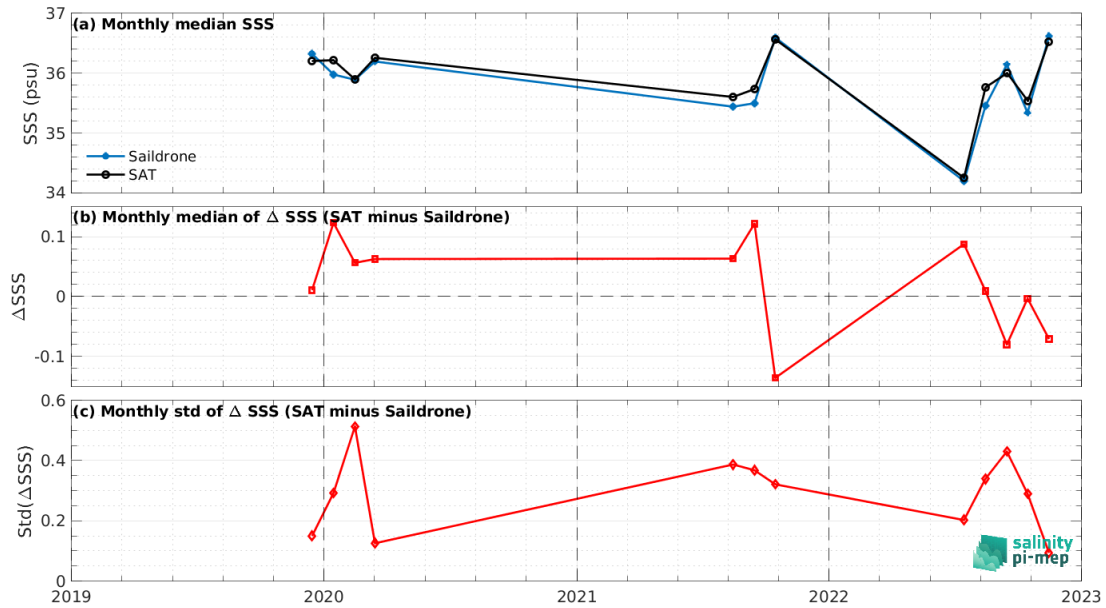
Figure 8: Time series of the monthly median SSS (top), median of \Delta\text{SSS} (Satellite - Sailldrone) and Std of \Delta\text{SSS} (Satellite - Sailldrone) over the Amazon and Orinoco river plumes Pi-MEP region considering all match-ups collected by the Pi-MEP.
