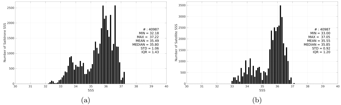
Figure 3: Histograms of SSS from Saildrone (a) and CCI SSS L4 Merged-OI v5.5 - 30-day running (ESA) (b) considering all match-up pairs per bins of 0.1 over the Amazon and Orinoco river plumes Pi-MEP region and for the full satellite product period.
