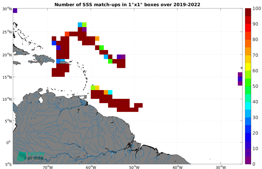
Figure 5: Number of SSS match-ups between Saildrone SSS and the CCI SSS L4 Merged-OI v5.5 - 30-day running (ESA) SSS product for the Amazon and Orinoco river plumes Pi-MEP region over 1^\circ \times 1^\circ boxes and for the full satellite product period.
