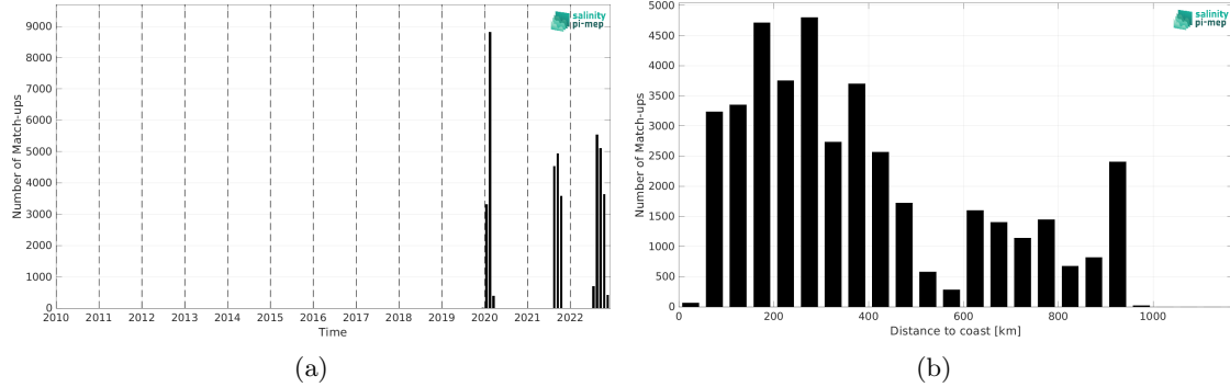
Figure 2: Number of match-ups between Saildrone and CCI SSS L4 Merged-OI v5.5 - 30-day running (ESA) SSS as a function of time (a) and as function of the distance to coast (b) over the Amazon and Orinoco river plumes Pi-MEP region and for the full satellite product period.
