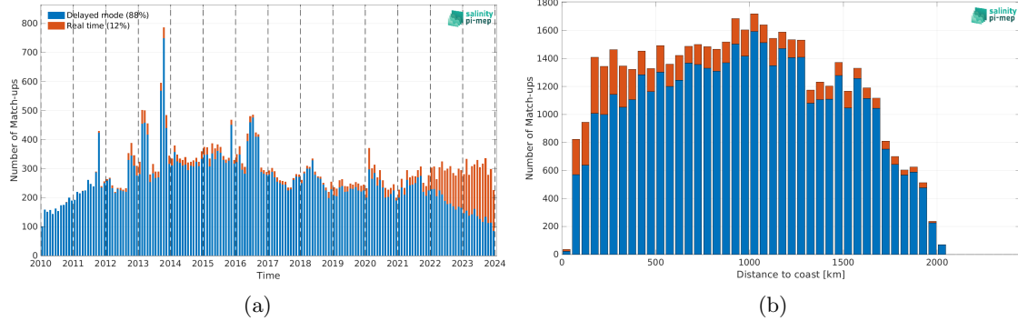
Figure 2: Number of match-ups between Argo and CCI SSS L4 Merged-OI v5.5 - 30-day running (ESA) SSS as a function of time (a) and as function of the distance to coast (b) over the Amazon and Orinoco river plumes Pi-MEP region and for the full satellite product period.
