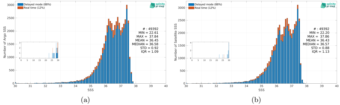
Figure 3: Histograms of SSS from Argo (a) and CCI SSS L4 Merged-OI v5.5 - 30-day running (ESA) (b) considering all match-up pairs per bins of 0.1 over the Amazon and Orinoco river plumes Pi-MEP region and for the full satellite product period.
