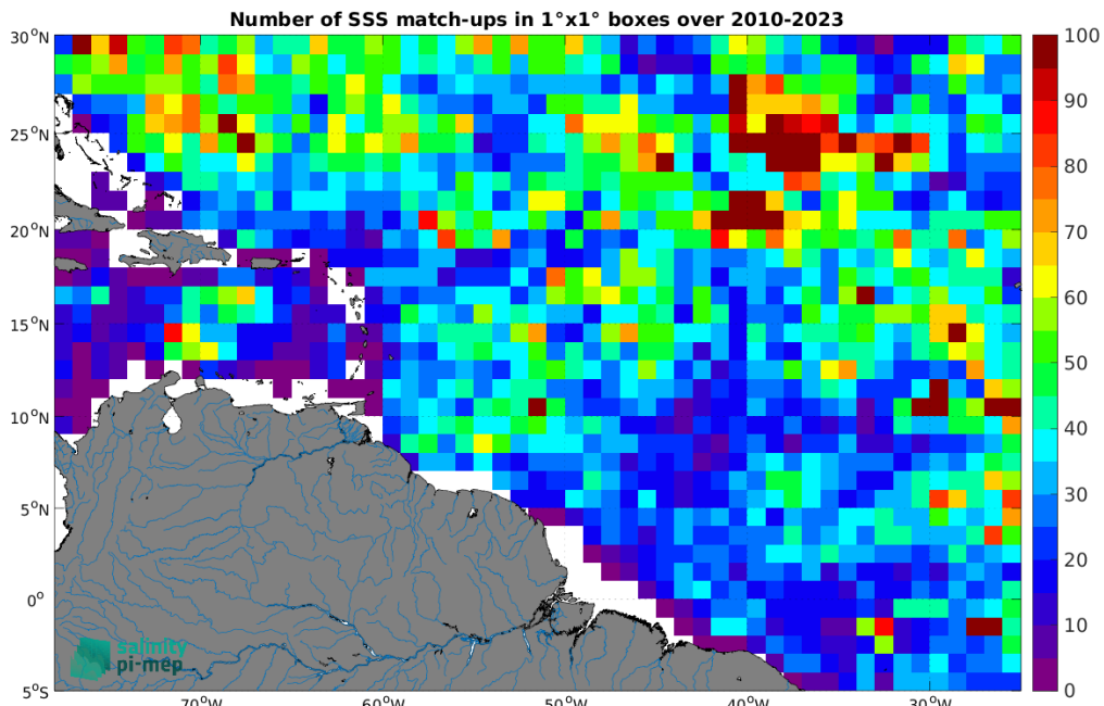
Figure 5: Number of SSS match-ups between Argo SSS and the CCI SSS L4 Merged-OI v5.5 - 30-day running (ESA) SSS product for the Amazon and Orinoco river plumes Pi-MEP region over 1^\circ \times 1^\circ boxes and for the full satellite product period.
