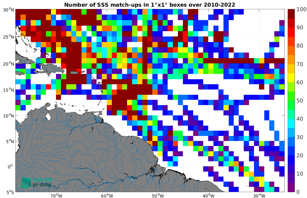
Figure 5: Number of SSS match-ups between TSG (SAMOS) SSS and the CCI SSS L4 Merged-OI v4.41 - 7-day running (ESA) SSS product for the Amazon and Orinoco river plumes Pi-MEP region over 1^\circ \times 1^\circ boxes and for the full satellite product period.
