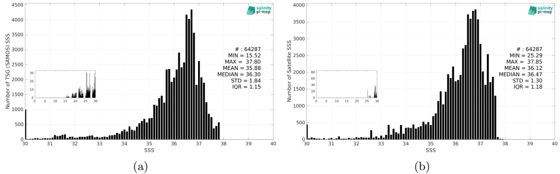
Figure 3: Histograms of SSS from TSG (SAMOS) (a) and CCI SSS L4 Merged-OI v4.41 - 7-day running (ESA) (b) considering all match-up pairs per bins of 0.1 over the Amazon and Orinoco river plumes Pi-MEP region and for the full satellite product period.
