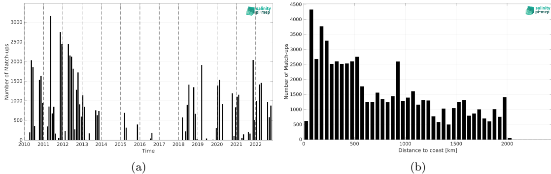
Figure 2: Number of match-ups between TSG (SAMOS) and CCI SSS L4 Merged-OI v4.41 - 7-day running (ESA) SSS as a function of time (a) and as function of the distance to coast (b) over the Amazon and Orinoco river plumes Pi-MEP region and for the full satellite product period.
