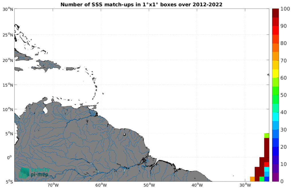
Figure 5: Number of SSS match-ups between TSG (Polarstern) SSS and the CCI SSS L4 Merged-OI v4.41 - 7-day running (ESA) SSS product for the Amazon and Orinoco river plumes Pi-MEP region over 1^\circ \times 1^\circ boxes and for the full satellite product period.
