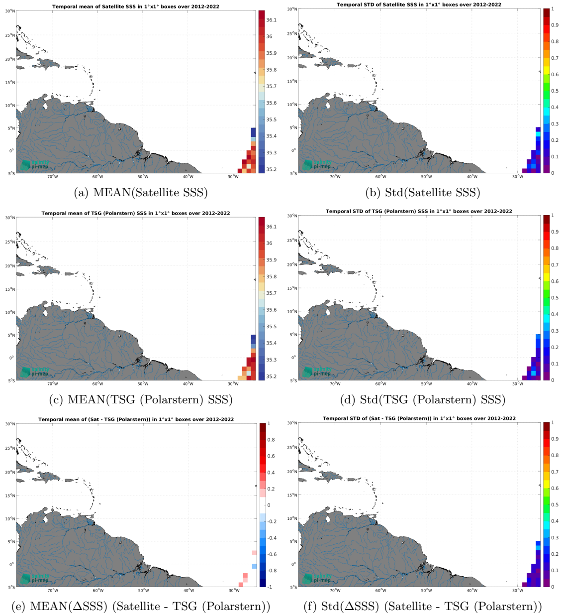
Figure 7: Temporal mean (left) and Std (right) of SSS from CCI SSS L4 Merged-OI v4.41 - 7-day running (ESA) (top), TSG (Polarstern) (middle), and of \Delta SSS (Satellite - TSG (Polarstern)). Only match-up pairs are used to generate these maps.
