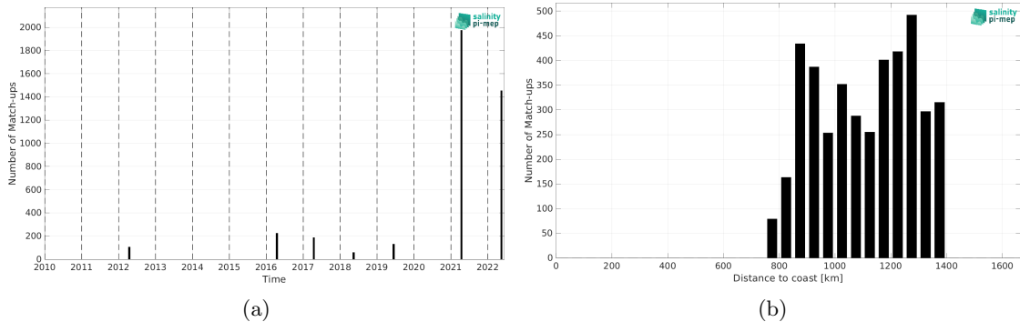
Figure 2: Number of match-ups between TSG (Polarstern) and CCI SSS L4 Merged-OI v4.41 - 7-day running (ESA) SSS as a function of time (a) and as function of the distance to coast (b) over the Amazon and Orinoco river plumes Pi-MEP region and for the full satellite product period.
