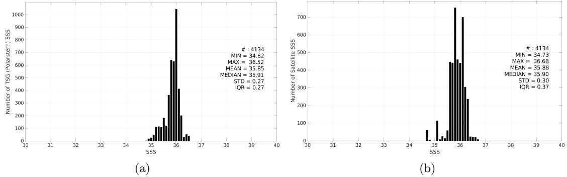
Figure 3: Histograms of SSS from TSG (Polarstern) (a) and CCI SSS L4 Merged-OI v4.41 - 7-day running (ESA) (b) considering all match-up pairs per bins of 0.1 over the Amazon and Orinoco river plumes Pi-MEP region and for the full satellite product period.
