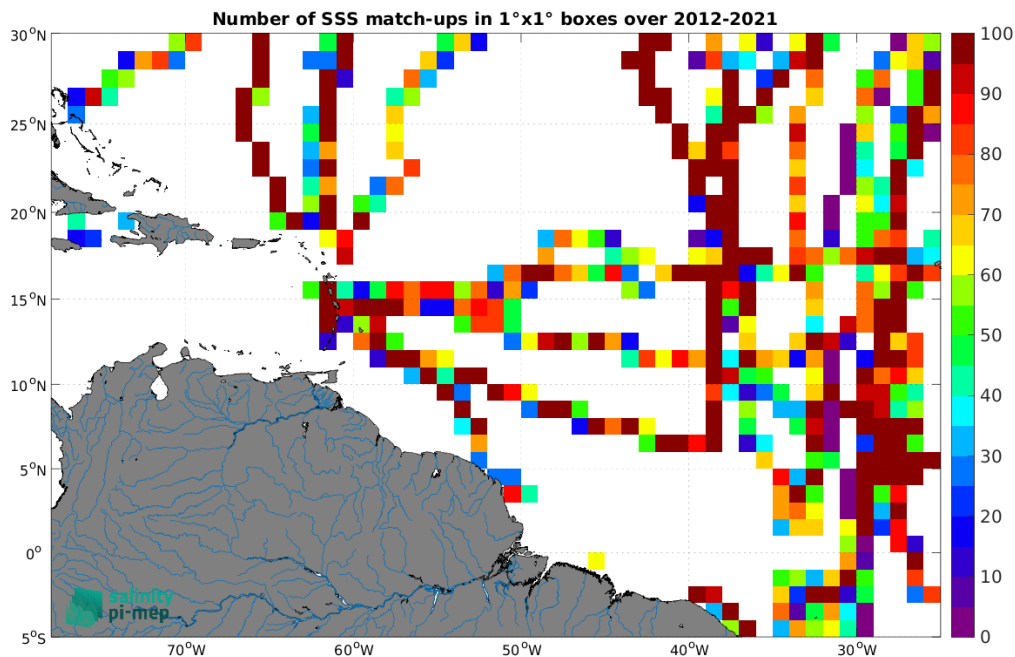
Figure 5: Number of SSS match-ups between TSG (GOSUD-Sailing-ship) SSS and the CCI SSS L4 Merged-OI v4.41 - 7-day running (ESA) SSS product for the Amazon and Orinoco river plumes Pi-MEP region over 1^\circ \times 1^\circ boxes and for the full satellite product period.
