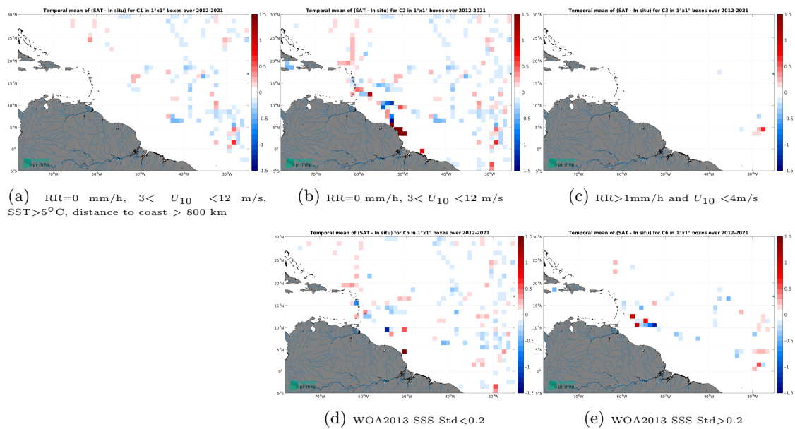
Figure 14: Temporal mean gridded over spatial boxes of size 1^\circ \times 1^\circ of \Delta SSS (CCI SSS L4 Merged-OI v4.41 - 7-day running (ESA) - TSG (GOSUD-Sailing-ship)) for 5 different subdatasets corresponding to:RR=0 mm/h, 3 < U_{10} < 12 m/s, SST >5^\circ\text{C} , distance to coast > 800 km (a), RR=0 mm/h, 3 < U_{10} < 12 m/s (b), RR >1 mm/h and U_{10} < 4 m/s (c), WOA2013 SSS Std <0.2 (d), WOA2013 SSS Std >0.2 (e).
