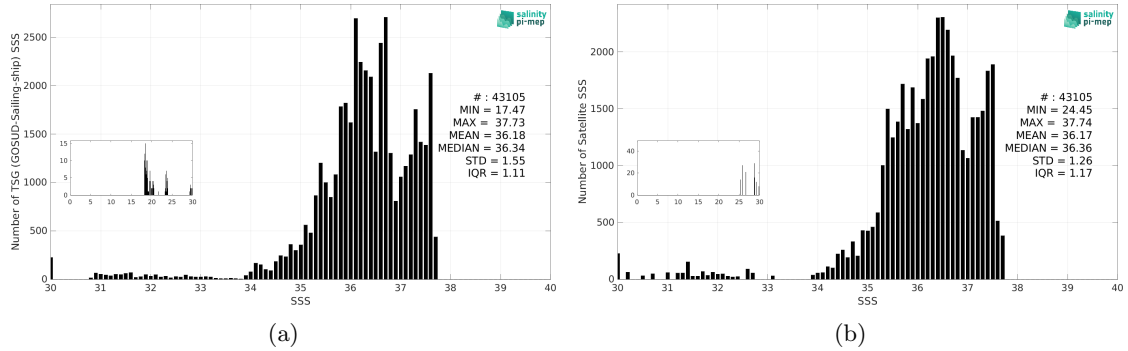
Figure 3: Histograms of SSS from TSG (GOSUD-Sailing-ship) (a) and CCI SSS L4 Merged-OI v4.41 - 7-day running (ESA) (b) considering all match-up pairs per bins of 0.1 over the Amazon and Orinoco river plumes Pi-MEP region and for the full satellite product period.
