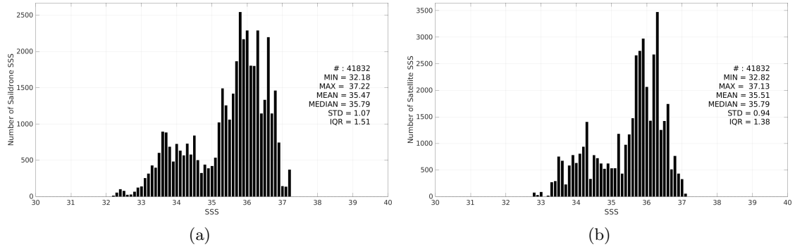
Figure 3: Histograms of SSS from Saildrone (a) and CCI SSS L4 Merged-OI v4.41 - 7-day running (ESA) (b) considering all match-up pairs per bins of 0.1 over the Amazon and Orinoco river plumes Pi-MEP region and for the full satellite product period.
