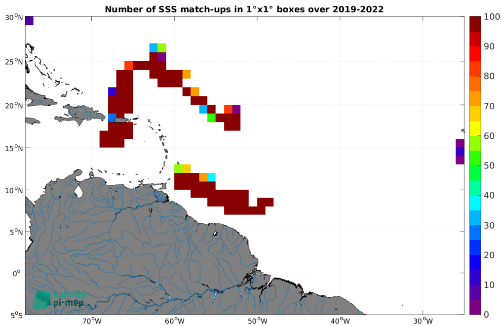
Figure 5: Number of SSS match-ups between Saildrone SSS and the CCI SSS L4 Merged-OI v4.41 - 7-day running (ESA) SSS product for the Amazon and Orinoco river plumes Pi-MEP region over 1^\circ \times 1^\circ boxes and for the full satellite product period.
