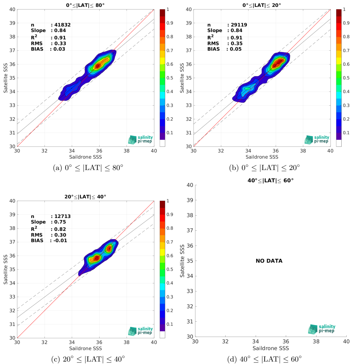
Figure 10: Contour maps of the concentration of CCI SSS L4 Merged-OI v4.41 - 7-day running (ESA) SSS (y-axis) versus Saildrone SSS (x-axis) at match-up pairs for different latitude bands. For each plot, the red line shows x=y . The black thin and dashed lines indicate a linear fit through the data cloud and the \pm 95\% confidence levels, respectively. The number match-up pairs n , the slope and R^2 coefficient of the linear fit, the root mean square (RMS) and the mean bias between satellite and in situ data are indicated for each latitude band in each plots.
