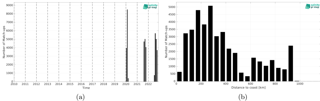
Figure 2: Number of match-ups between Saildrone and CCI SSS L4 Merged-OI v4.41 - 7-day running (ESA) SSS as a function of time (a) and as function of the distance to coast (b) over the Amazon and Orinoco river plumes Pi-MEP region and for the full satellite product period.
