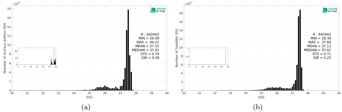
Figure 3: Histograms of SSS from Surface drifters (a) and CCI SSS L4 Merged-OI v4.41 - 7-day running (ESA) (b) considering all match-up pairs per bins of 0.1 over the Amazon and Orinoco river plumes Pi-MEP region and for the full satellite product period.
