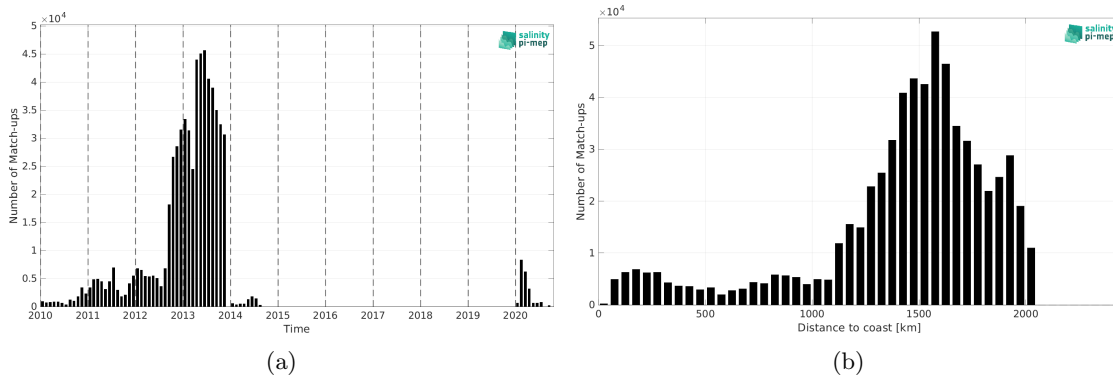
Figure 2: Number of match-ups between Surface drifters and CCI SSS L4 Merged-OI v4.41 - 7-day running (ESA) SSS as a function of time (a) and as function of the distance to coast (b) over the Amazon and Orinoco river plumes Pi-MEP region and for the full satellite product period.
