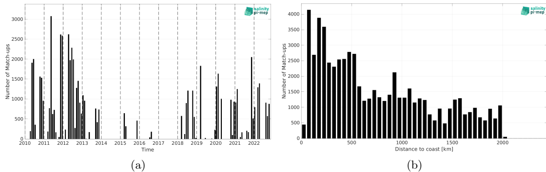
Figure 2: Number of match-ups between TSG (SAMOS) and CCI SSS L4 Merged-OI v4.41 - 30-day running (ESA) SSS as a function of time (a) and as function of the distance to coast (b) over the Amazon and Orinoco river plumes Pi-MEP region and for the full satellite product period.
