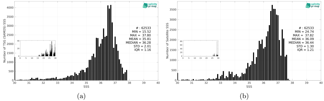
Figure 3: Histograms of SSS from TSG (SAMOS) (a) and CCI SSS L4 Merged-OI v4.41 - 30-day running (ESA) (b) considering all match-up pairs per bins of 0.1 over the Amazon and Orinoco river plumes Pi-MEP region and for the full satellite product period.
