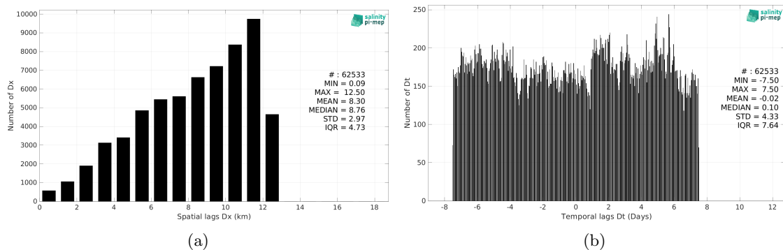
Figure 6: Histograms of the spatial (a) and temporal (b) lags between the location/time of the TSG (SAMOS) measurement and the date of the corresponding CCI SSS L4 Merged-OI v4.41 - 30-day running (ESA) SSS pixel.
