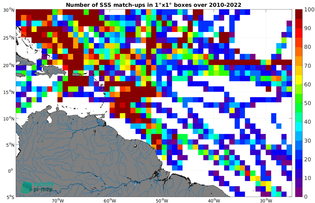
Figure 5: Number of SSS match-ups between TSG (SAMOS) SSS and the CCI SSS L4 Merged-OI v4.41 - 30-day running (ESA) SSS product for the Amazon and Orinoco river plumes Pi-MEP region over 1^\circ \times 1^\circ boxes and for the full satellite product period.
