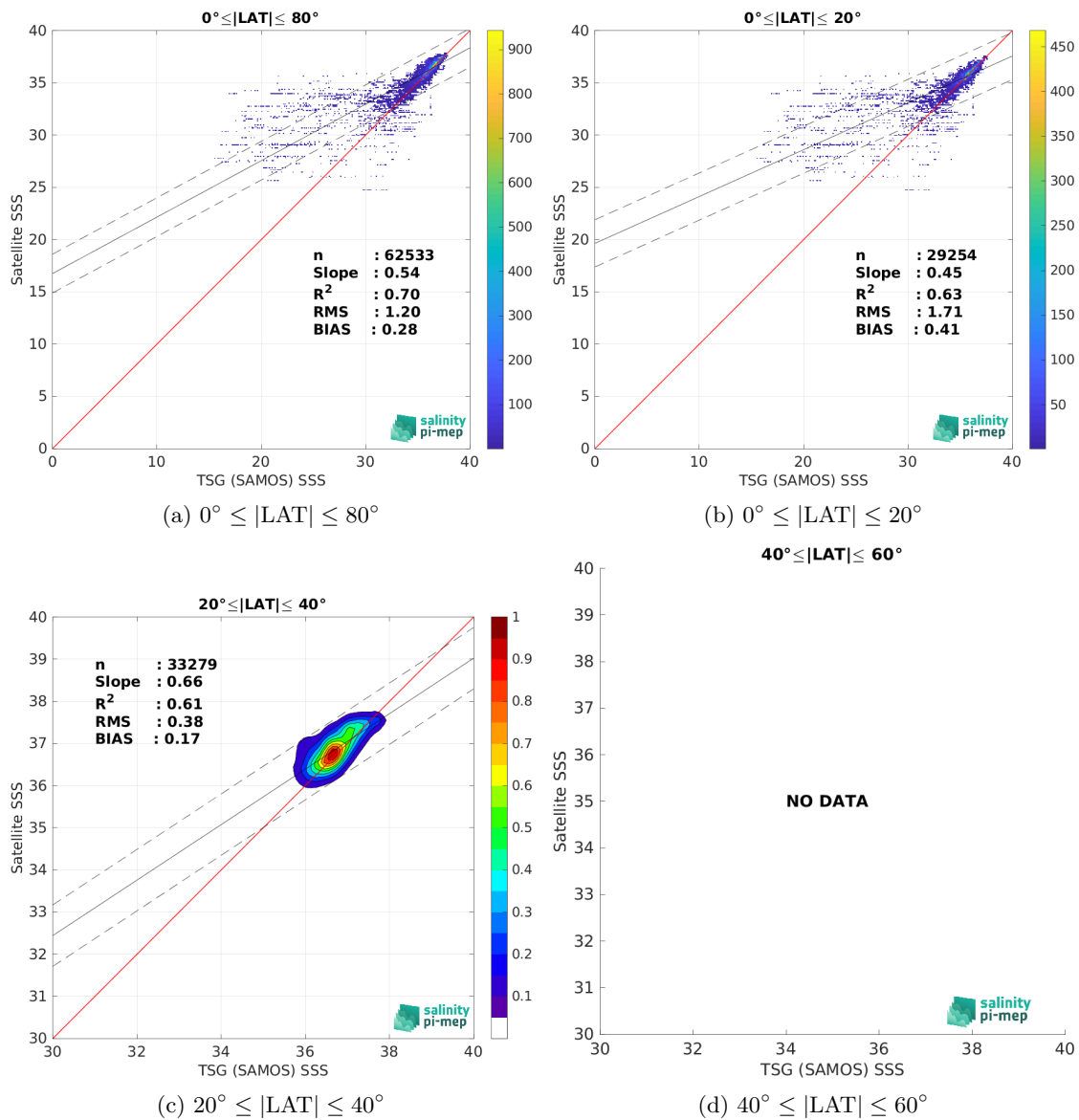
Figure 10: Contour maps of the concentration of CCI SSS L4 Merged-OI v4.41 - 30-day running (ESA) SSS (y-axis) versus TSG (SAMOS) SSS (x-axis) at match-up pairs for different latitude bands. For each plot, the red line shows x=y . The black thin and dashed lines indicate a linear fit through the data cloud and the \pm 95\% confidence levels, respectively. The number match-up pairs n , the slope and R^2 coefficient of the linear fit, the root mean square (RMS) and the mean bias between satellite and in situ data are indicated for each latitude band in each plots.
