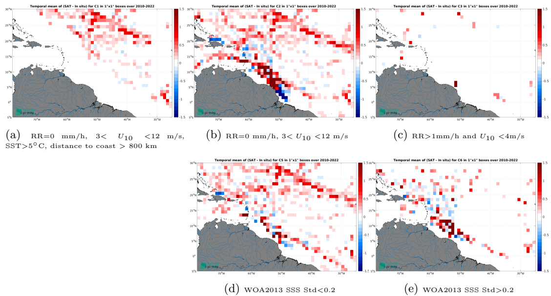
Figure 14: Temporal mean gridded over spatial boxes of size 1^\circ \times 1^\circ of \Delta\text{SSS} (CCI SSS L4 Merged-OI v4.41 - 30-day running (ESA) - TSG (SAMOS)) for 5 different subdatasets corresponding to:RR=0 mm/h, 3 < U_{10} < 12 m/s, SST >5^\circ\text{C} , distance to coast > 800 km (a), RR=0 mm/h, 3 < U_{10} < 12 m/s (b), RR >1 mm/h and U_{10} < 4 m/s (c), WOA2013 SSS Std <0.2 (d), WOA2013 SSS Std >0.2 (e).
