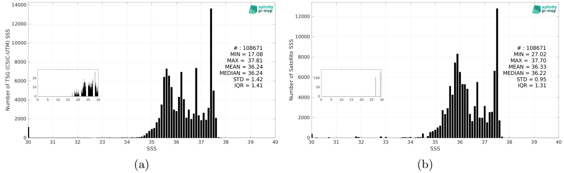
Figure 3: Histograms of SSS from TSG (CSIC-UTM) (a) and CCI SSS L4 Merged-OI v4.41 - 30-day running (ESA) (b) considering all match-up pairs per bins of 0.1 over the Amazon and Orinoco river plumes Pi-MEP region and for the full satellite product period.
