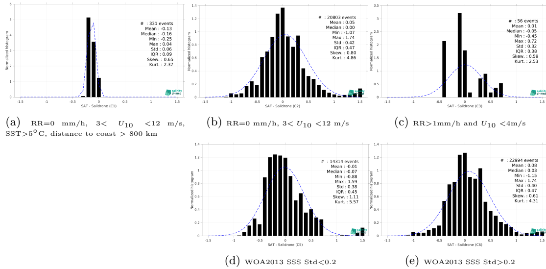
Figure 15: Normalized histogram of \Delta SSS (CCI SSS L4 Merged-OI v4.41 - 30-day running (ESA) - Saldrone) for 5 different subdatasets corresponding to: RR=0 mm/h, 3 < U_{10} < 12 m/s, SST>5°C, distance to coast > 800 km (a), RR=0 mm/h, 3 < U_{10} < 12 m/s (b), RR>1mm/h and U_{10} < 4 m/s (c), WOA2013 SSS Std<0.2 (d), WOA2013 SSS Std>0.2 (e).
