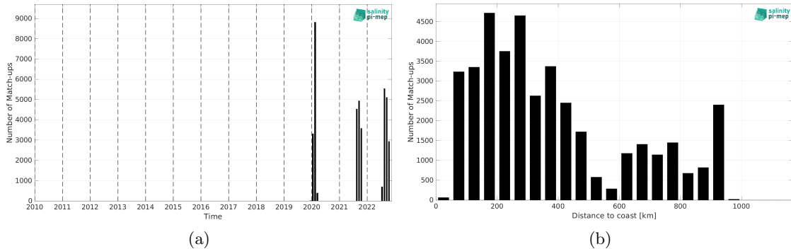
Figure 2: Number of match-ups between Saildrone and CCI SSS L4 Merged-OI v4.41 - 30-day running (ESA) SSS as a function of time (a) and as function of the distance to coast (b) over the Amazon and Orinoco river plumes Pi-MEP region and for the full satellite product period.
