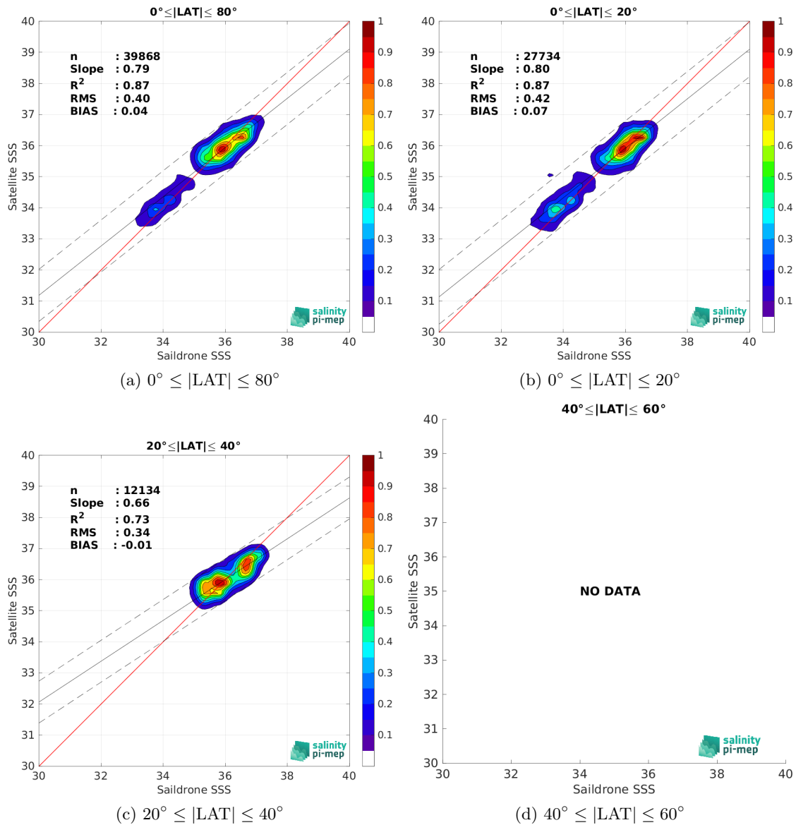
Figure 10: Contour maps of the concentration of CCI SSS L4 Merged-OI v4.41 - 30-day running (ESA) SSS (y-axis) versus Saldrone SSS (x-axis) at match-up pairs for different latitude bands. For each plot, the red line shows x=y . The black thin and dashed lines indicate a linear fit through the data cloud and the \pm 95\% confidence levels, respectively. The number match-up pairs n , the slope and R^2 coefficient of the linear fit, the root mean square (RMS) and the mean bias between satellite and in situ data are indicated for each latitude band in each plots.
