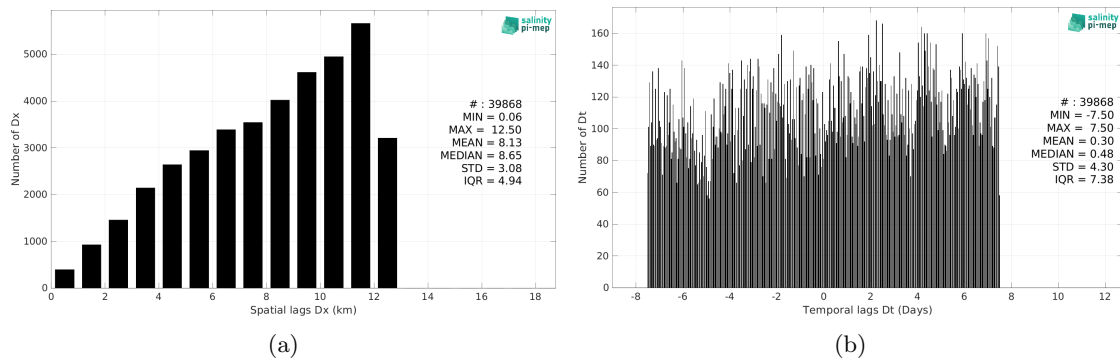
Figure 6: Histograms of the spatial (a) and temporal (b) lags between the location/time of the Sailldrone measurement and the date of the corresponding CCI SSS L4 Merged-OI v4.41 - 30-day running (ESA) SSS pixel.
