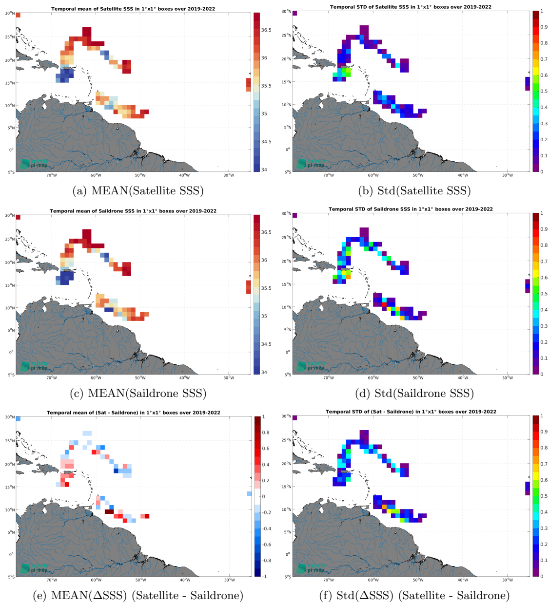
Figure 7: Temporal mean (left) and Std (right) of SSS from CCI SSS L4 Merged-OI v4.41 - 30-day running (ESA) (top), Saildrone (middle), and of \Delta SSS (Satellite - Saildrone). Only match-up pairs are used to generate these maps.
