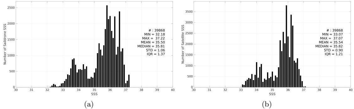
Figure 3: Histograms of SSS from Saildrone (a) and CCI SSS L4 Merged-OI v4.41 - 30-day running (ESA) (b) considering all match-up pairs per bins of 0.1 over the Amazon and Orinoco river plumes Pi-MEP region and for the full satellite product period.
