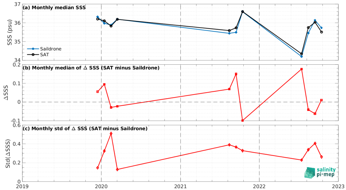
Figure 8: Time series of the monthly median SSS (top), median of \Delta SSS (Satellite - Sairdrone) and Std of \Delta SSS (Satellite - Sairdrone) over the Amazon and Orinoco river plumes Pi-MEP region considering all match-ups collected by the Pi-MEP.
