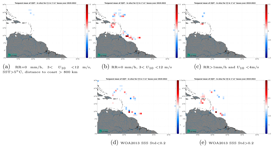
Figure 14: Temporal mean gridded over spatial boxes of size 1^\circ \times 1^\circ of \Delta SSS (CCI SSS L4 Merged-OI v4.41 - 30-day running (ESA) - Saildrone) for 5 different subdatasets corresponding to:RR=0 mm/h, 3 < U_{10} < 12 m/s, SST >5^\circ C, distance to coast > 800 km (a), RR=0 mm/h, 3 < U_{10} < 12 m/s (b), RR >1 mm/h and U_{10} < 4 m/s (c), WOA2013 SSS Std <0.2 (d), WOA2013 SSS Std >0.2 (e).
