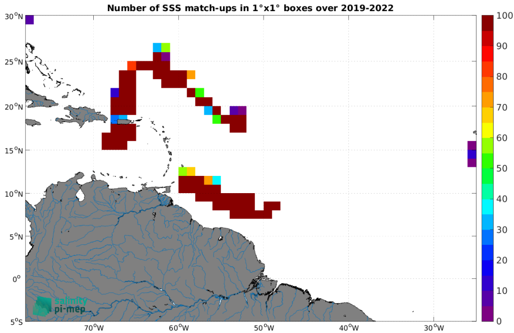
Figure 5: Number of SSS match-ups between Saildrone SSS and the CCI SSS L4 Merged-OI v4.41 - 30-day running (ESA) SSS product for the Amazon and Orinoco river plumes Pi-MEP region over 1^\circ \times 1^\circ boxes and for the full satellite product period.
