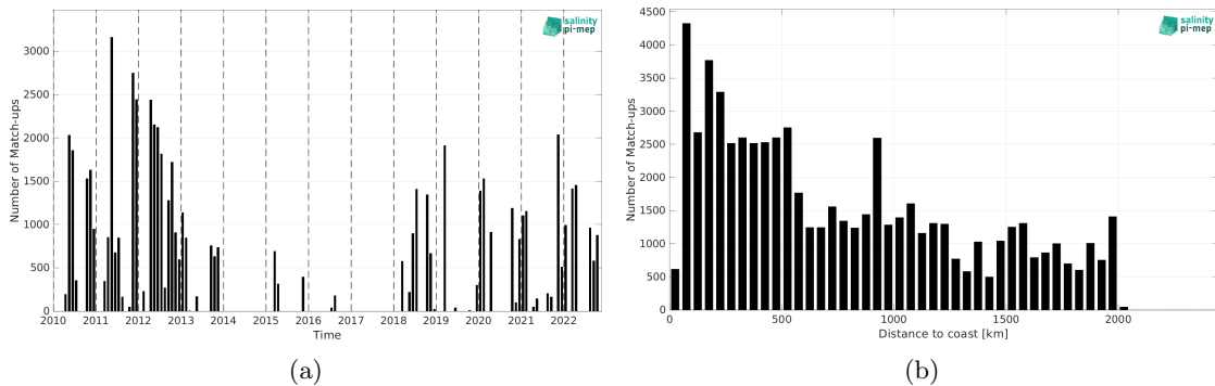
Figure 1: Number of match-ups between TSG (SAMOS) and CCI SSS L4 Merged-OI v4.4 - 7-day running (ESA) SSS as a function of time (a) and as function of the distance to coast (b) over the Amazon and Orinoco river plumes Pi-MEP region and for the full satellite product period.
