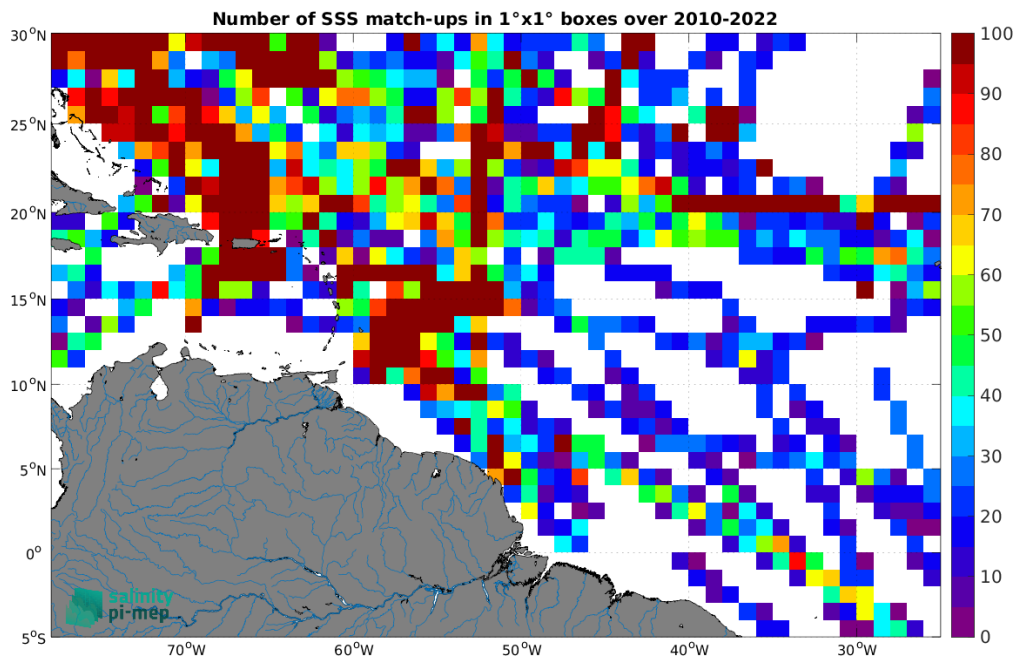
Figure 4: Number of SSS match-ups between TSG (SAMOS) SSS and the CCI SSS L4 Merged-OI v4.4 - 7-day running (ESA) SSS product for the Amazon and Orinoco river plumes Pi-MEP region over 1^\circ \times 1^\circ boxes and for the full satellite product period.
