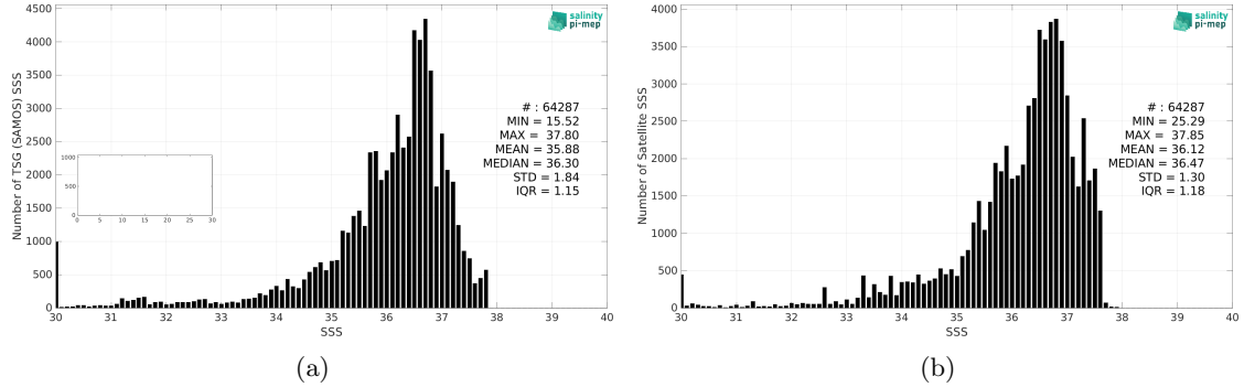
Figure 2: Histograms of SSS from TSG (SAMOS) (a) and CCI SSS L4 Merged-OI v4.4 - 7-day running (ESA) (b) considering all match-up pairs per bins of 0.1 over the Amazon and Orinoco river plumes Pi-MEP region and for the full satellite product period.
