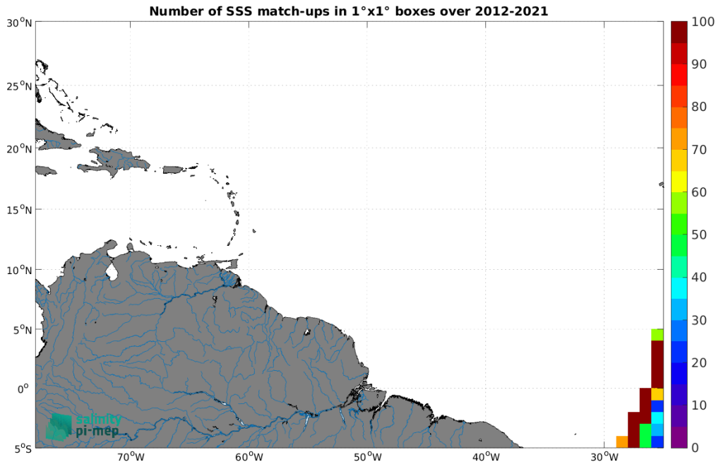
Figure 4: Number of SSS match-ups between TSG (Polarstern) SSS and the CCI SSS L4 Merged-OI v4.4 - 7-day running (ESA) SSS product for the Amazon and Orinoco river plumes Pi-MEP region over 1^\circ \times 1^\circ boxes and for the full satellite product period.
