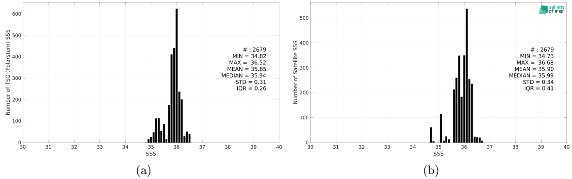
Figure 2: Histograms of SSS from TSG (Polarstern) (a) and CCI SSS L4 Merged-OI v4.4 - 7-day running (ESA) (b) considering all match-up pairs per bins of 0.1 over the Amazon and Orinoco river plumes Pi-MEP region and for the full satellite product period.
