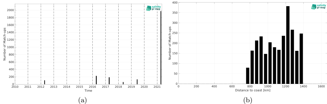
Figure 1: Number of match-ups between TSG (Polarstern) and CCI SSS L4 Merged-OI v4.4 - 7-day running (ESA) SSS as a function of time (a) and as function of the distance to coast (b) over the Amazon and Orinoco river plumes Pi-MEP region and for the full satellite product period.
