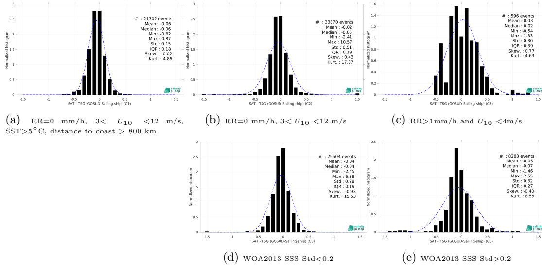
Figure 13: Normalized histogram of \Delta\text{SSS} (CCI SSS L4 Merged-OI v4.4 - 7-day running (ESA) - TSG (GOSUD-Sailing-ship)) for 5 different subdatasets corresponding to: RR=0 mm/h, 3 < U_{10} < 12 m/s, SST>5°C, distance to coast > 800 km (a), RR=0 mm/h, 3 < U_{10} < 12 m/s (b), RR>1mm/h and U_{10} < 4 m/s (c), WOA2013 SSS Std<0.2 (d), WOA2013 SSS Std>0.2 (e).
