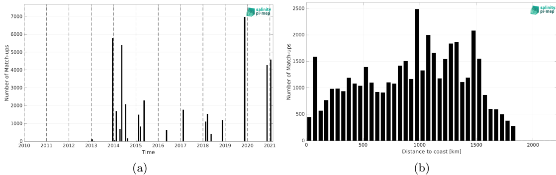
Figure 1: Number of match-ups between TSG (GOSUD-Sailing-ship) and CCI SSS L4 Merged-OI v4.4 - 7-day running (ESA) SSS as a function of time (a) and as function of the distance to coast (b) over the Amazon and Orinoco river plumes Pi-MEP region and for the full satellite product period.
