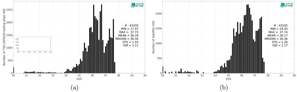
Figure 2: Histograms of SSS from TSG (GOSUD-Sailing-ship) (a) and CCI SSS L4 Merged-OI v4.4 - 7-day running (ESA) (b) considering all match-up pairs per bins of 0.1 over the Amazon and Orinoco river plumes Pi-MEP region and for the full satellite product period.
