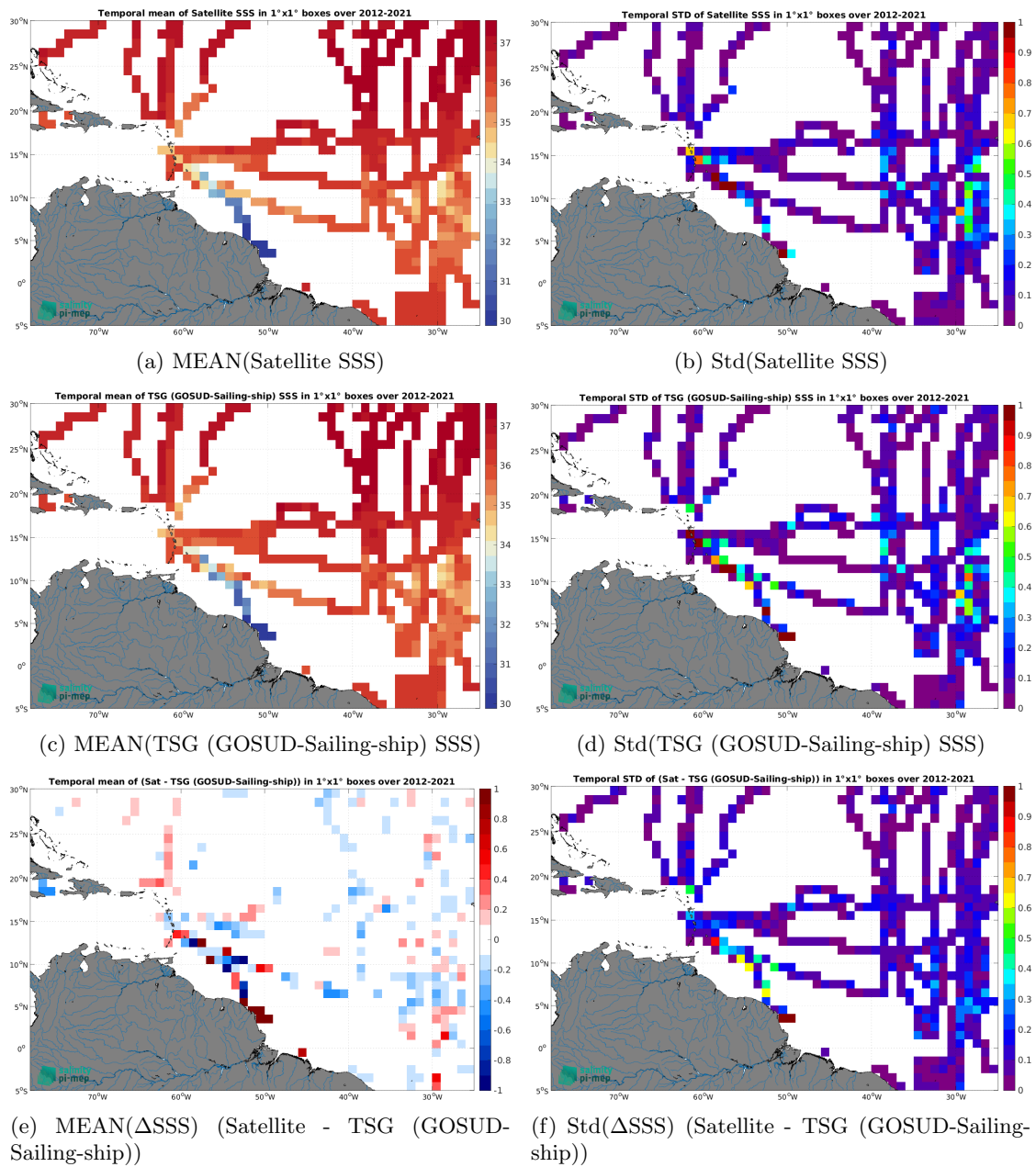
Figure 6: Temporal mean (left) and Std (right) of SSS from CCI SSS L4 Merged-OI v4.4 - 7-day running (ESA) (top), TSG (GOSUD-Sailing-ship) (middle), and of \Delta SSS (Satellite - TSG (GOSUD-Sailing-ship)). Only match-up pairs are used to generate these maps.
