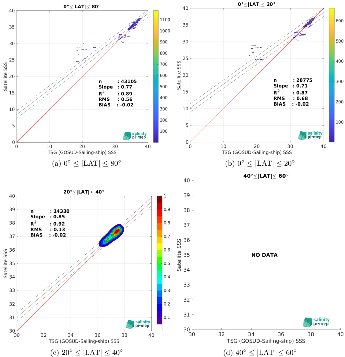
Figure 9: Contour maps of the concentration of CCI SSS L4 Merged-OI v4.4 - 7-day running (ESA) SSS (y-axis) versus TSG (GOSUD-Sailing-ship) SSS (x-axis) at match-up pairs for different latitude bands. For each plot, the red line shows x=y . The black thin and dashed lines indicate a linear fit through the data cloud and the \pm 95\% confidence levels, respectively. The number match-up pairs n , the slope and R^2 coefficient of the linear fit, the root mean square (RMS) and the mean bias between satellite and in situ data are indicated for each latitude band in each plots.
