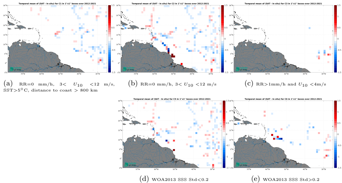
Figure 12: Temporal mean gridded over spatial boxes of size 1^\circ \times 1^\circ of \Delta SSS (CCI SSS L4 Merged-OI v4.4 - 7-day running (ESA) - TSG (GOSUD-Sailing-ship)) for 5 different subdatasets corresponding to:RR=0 mm/h, 3 < U_{10} < 12 m/s, SST >5^\circ\text{C} , distance to coast > 800 km (a), RR=0 mm/h, 3 < U_{10} < 12 m/s (b), RR >1 mm/h and U_{10} < 4 m/s (c), WOA2013 SSS Std <0.2 (d), WOA2013 SSS Std >0.2 (e).
