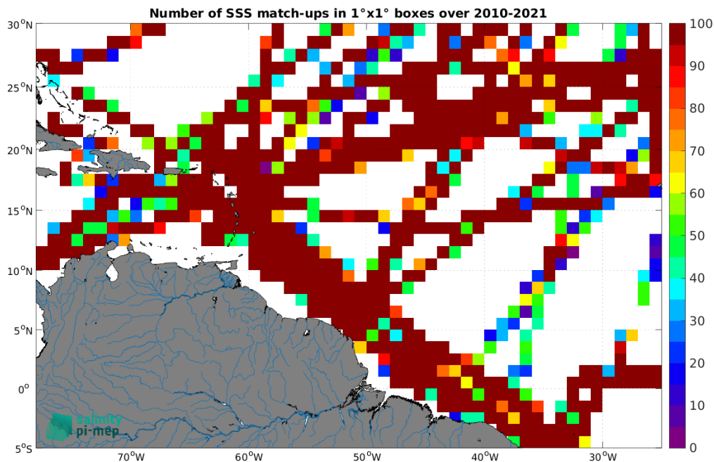
Figure 4: Number of SSS match-ups between TSG (GOSUD-Research-vessel) SSS and the CCI SSS L4 Merged-OI v4.4 - 7-day running (ESA) SSS product for the Amazon and Orinoco river plumes Pi-MEP region over 1^\circ \times 1^\circ boxes and for the full satellite product period.
