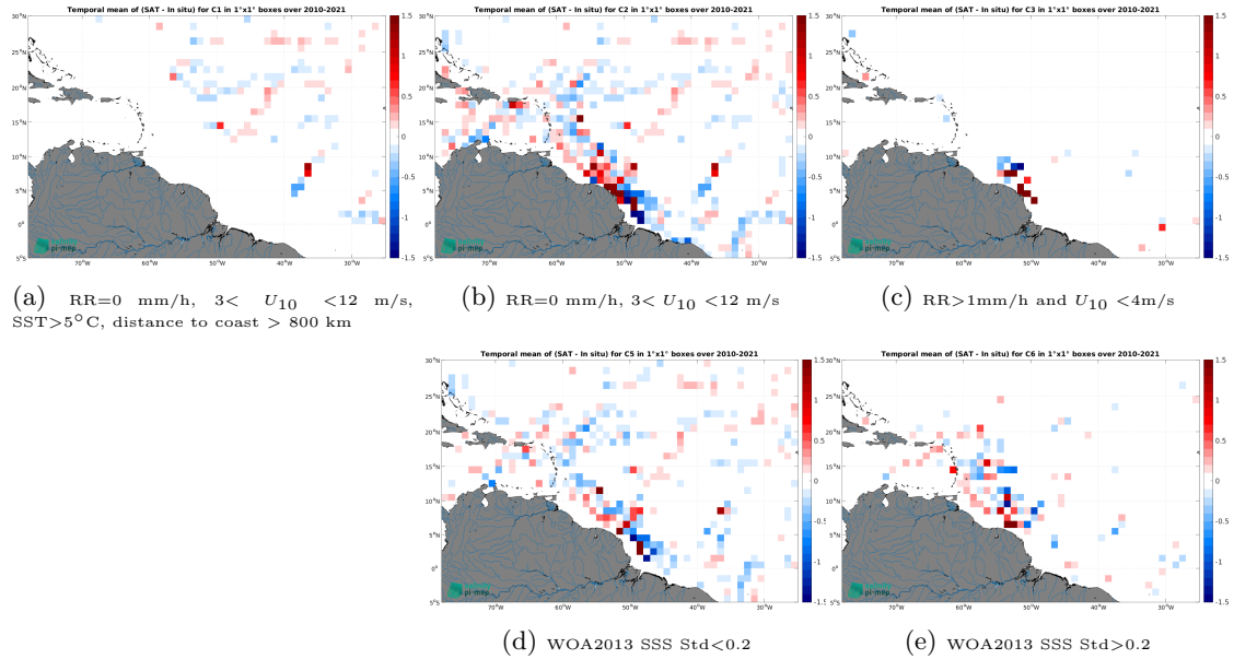
Figure 12: Temporal mean gridded over spatial boxes of size 1^{\circ}\times 1^{\circ} of \Delta SSS (CCI SSS L4 Merged-OI v4.4 - 7-day running (ESA) - TSG (GOSUD-Research-vessel)) for 5 different subdatasets corresponding to:RR=0 mm/h, 3 < U_{10} < 12 m/s, SST >5^{\circ}\text{C} , distance to coast > 800 km (a), RR=0 mm/h, 3 < U_{10} < 12 m/s (b), RR >1 mm/h and U_{10} < 4 m/s (c), WOA2013 SSS Std <0.2 (d), WOA2013 SSS Std >0.2 (e).
