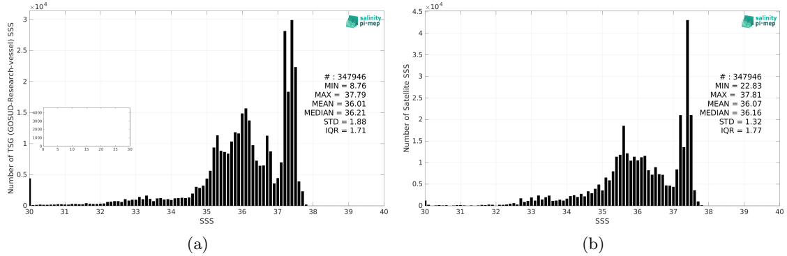
Figure 2: Histograms of SSS from TSG (GOSUD-Research-vessel) (a) and CCI SSS L4 Merged-OI v4.4 - 7-day running (ESA) (b) considering all match-up pairs per bins of 0.1 over the Amazon and Orinoco river plumes Pi-MEP region and for the full satellite product period.
