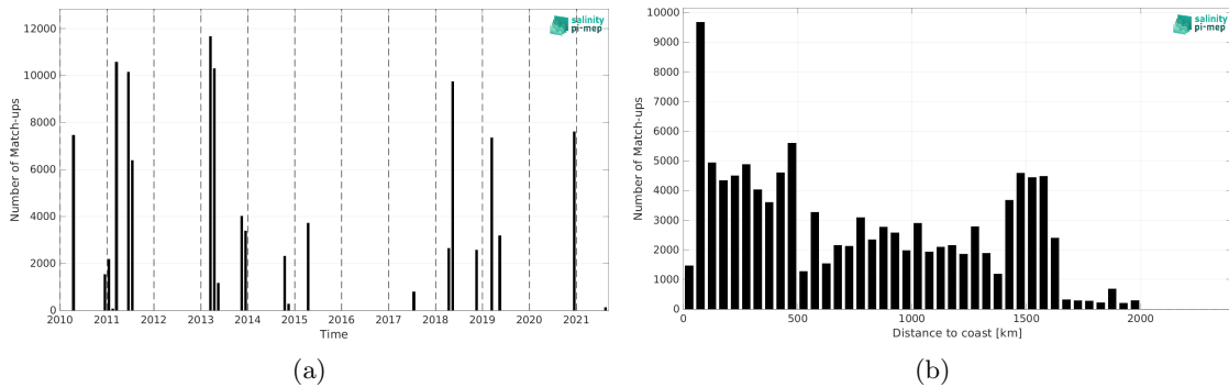
Figure 1: Number of match-ups between TSG (CSIC-UTM) and CCI SSS L4 Merged-OI v4.4 - 7-day running (ESA) SSS as a function of time (a) and as function of the distance to coast (b) over the Amazon and Orinoco river plumes Pi-MEP region and for the full satellite product period.
