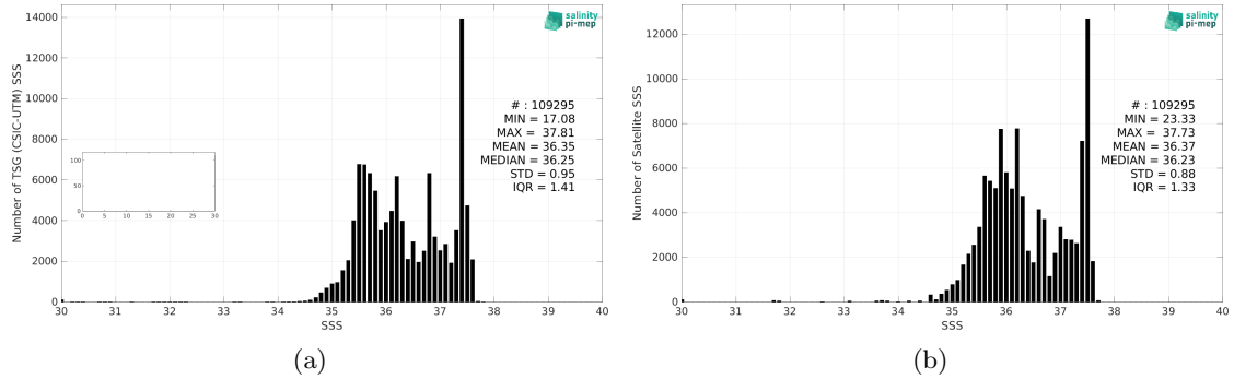
Figure 2: Histograms of SSS from TSG (CSIC-UTM) (a) and CCI SSS L4 Merged-OI v4.4 - 7-day running (ESA) (b) considering all match-up pairs per bins of 0.1 over the Amazon and Orinoco river plumes Pi-MEP region and for the full satellite product period.
