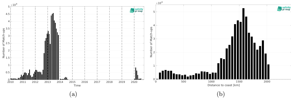
Figure 1: Number of match-ups between Surface drifters and CCI SSS L4 Merged-OI v4.4 - 7-day running (ESA) SSS as a function of time (a) and as function of the distance to coast (b) over the Amazon and Orinoco river plumes Pi-MEP region and for the full satellite product period.
