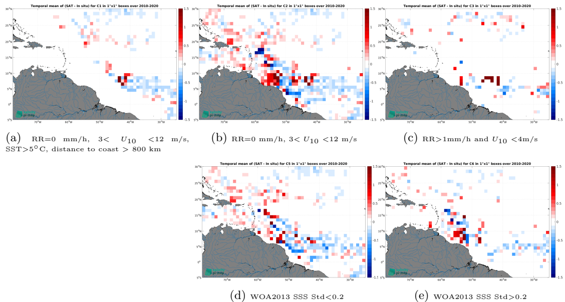
Figure 11: Temporal mean gridded over spatial boxes of size 1^\circ \times 1^\circ of \Delta SSS (CCI SSS L4 Merged-OI v4.4 - 7-day running (ESA) - Surface drifters) for 5 different subdatasets corresponding to:RR=0 mm/h, 3 < U_{10} < 12 m/s, SST >5^\circ C, distance to coast > 800 km (a), RR=0 mm/h, 3 < U_{10} < 12 m/s (b), RR >1 mm/h and U_{10} < 4 m/s (c), WOA2013 SSS Std <0.2 (d), WOA2013 SSS Std >0.2 (e).
