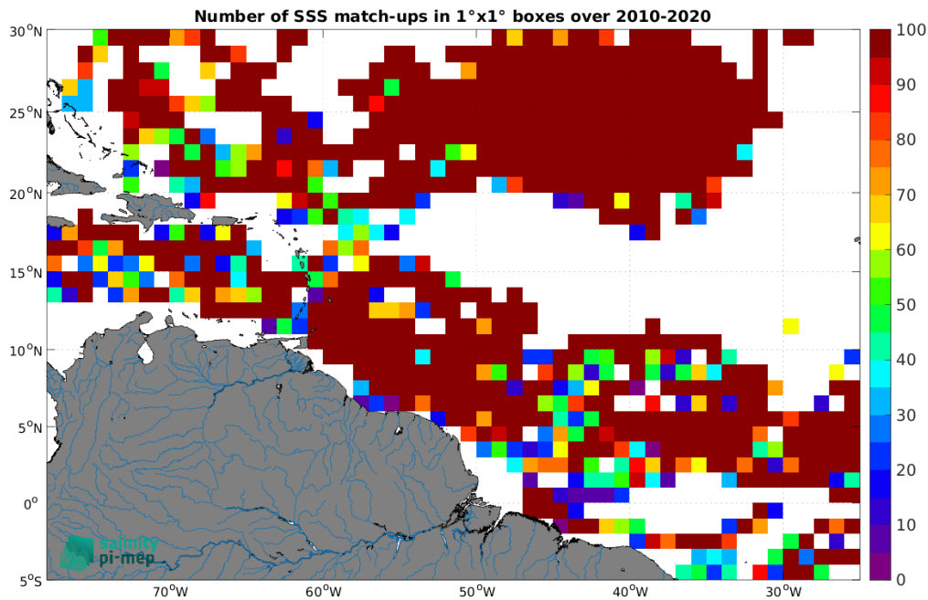
Figure 3: Number of SSS match-ups between Surface drifters SSS and the CCI SSS L4 Merged-OI v4.4 - 7-day running (ESA) SSS product for the Amazon and Orinoco river plumes Pi-MEP region over 1^{\circ} \times 1^{\circ} boxes and for the full satellite product period.
