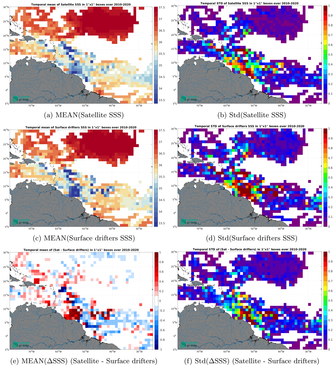
Figure 5: Temporal mean (left) and Std (right) of SSS from CCI SSS L4 Merged-OI v4.4 - 7-day running (ESA) (top), Surface drifters (middle), and of \Delta SSS (Satellite - Surface drifters). Only match-up pairs are used to generate these maps.
