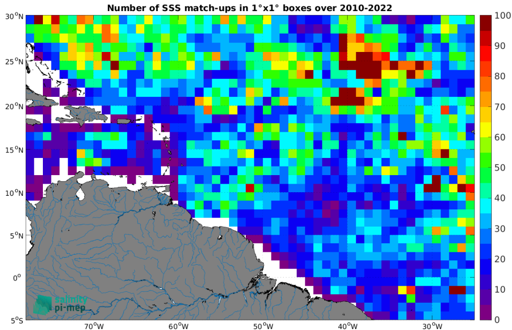
Figure 4: Number of SSS match-ups between Argo SSS and the CCI SSS L4 Merged-OI v4.4 - 7-day running (ESA) SSS product for the Amazon and Orinoco river plumes Pi-MEP region over 1^{\circ} \times 1^{\circ} boxes and for the full satellite product period.
