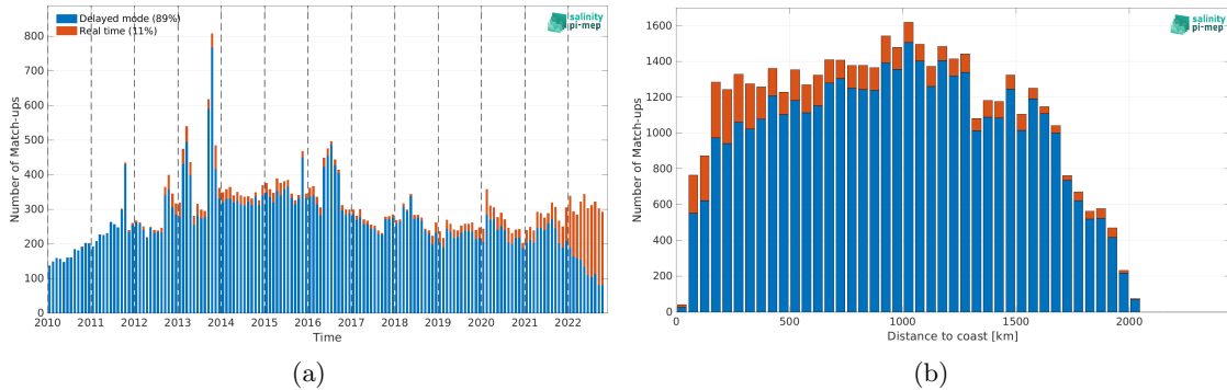
Figure 1: Number of match-ups between Argo and CCI SSS L4 Merged-OI v4.4 - 7-day running (ESA) SSS as a function of time (a) and as function of the distance to coast (b) over the Amazon and Orinoco river plumes Pi-MEP region and for the full satellite product period.
