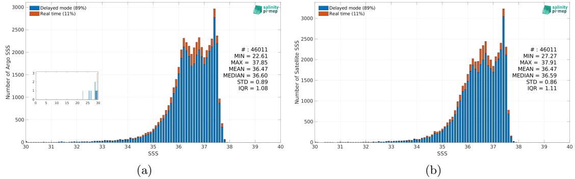
Figure 2: Histograms of SSS from Argo (a) and CCI SSS L4 Merged-OI v4.4 - 7-day running (ESA) (b) considering all match-up pairs per bins of 0.1 over the Amazon and Orinoco river plumes Pi-MEP region and for the full satellite product period.
