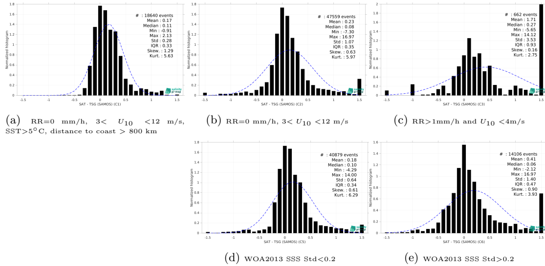
Figure 13: Normalized histogram of \Delta\text{SSS} (CCI SSS L4 Merged-OI v4.4 - 30-day running (ESA) - TSG (SAMOS)) for 5 different subdatasets corresponding to: RR=0 mm/h, 3 < U_{10} < 12 m/s, SST>5°C, distance to coast > 800 km (a), RR=0 mm/h, 3 < U_{10} < 12 m/s (b), RR>1mm/h and U_{10} < 4 m/s (c), WOA2013 SSS Std<0.2 (d), WOA2013 SSS Std>0.2 (e).
