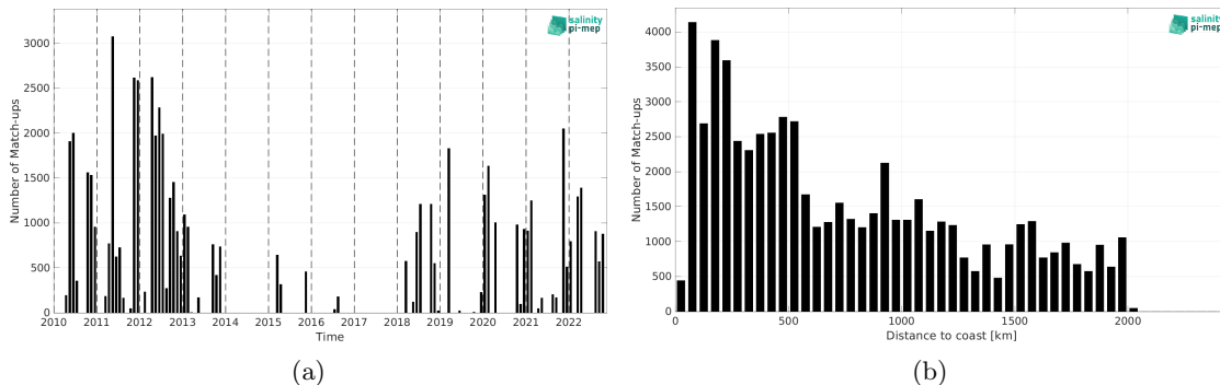
Figure 1: Number of match-ups between TSG (SAMOS) and CCI SSS L4 Merged-OI v4.4 - 30-day running (ESA) SSS as a function of time (a) and as function of the distance to coast (b) over the Amazon and Orinoco river plumes Pi-MEP region and for the full satellite product period.
