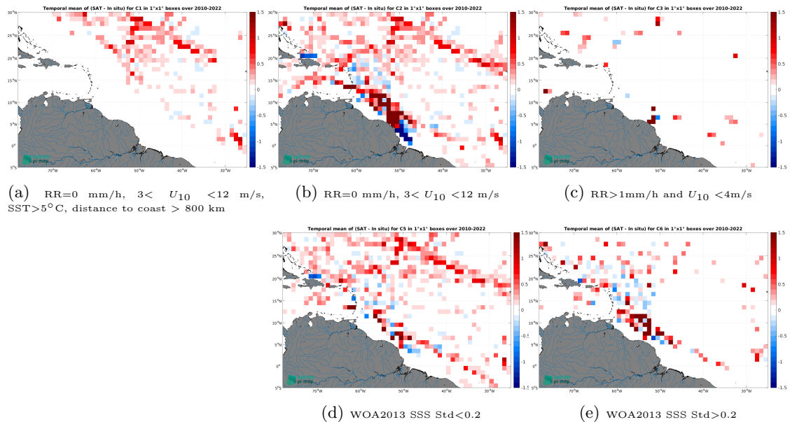
Figure 12: Temporal mean gridded over spatial boxes of size 1^\circ \times 1^\circ of \Delta SSS (CCI SSS L4 Merged-OI v4.4 - 30-day running (ESA) - TSG (SAMOS)) for 5 different subdatasets corresponding to:RR=0 mm/h, 3 < U_{10} < 12 m/s, SST >5^\circ\text{C} , distance to coast > 800 km (a), RR=0 mm/h, 3 < U_{10} < 12 m/s (b), RR >1 mm/h and U_{10} < 4 m/s (c), WOA2013 SSS Std <0.2 (d), WOA2013 SSS Std >0.2 (e).
