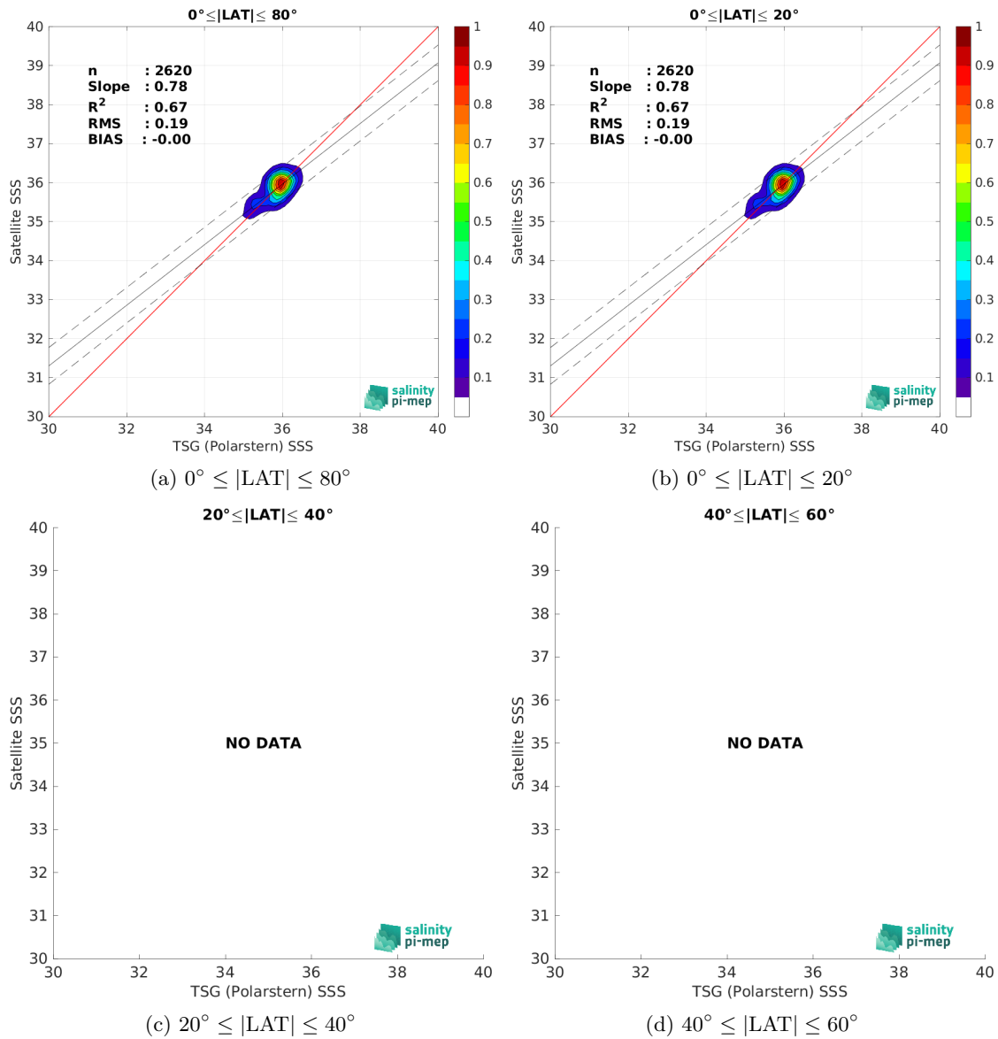
Figure 9: Contour maps of the concentration of CCI SSS L4 Merged-OI v4.4 - 30-day running (ESA) SSS ( y -axis) versus TSG (Polarstern) SSS ( x -axis) at match-up pairs for different latitude bands. For each plot, the red line shows x=y . The black thin and dashed lines indicate a linear fit through the data cloud and the \pm 95\% confidence levels, respectively. The number match-up pairs n , the slope and R^2 coefficient of the linear fit, the root mean square (RMS) and the mean bias between satellite and in situ data are indicated for each latitude band in each plots.
