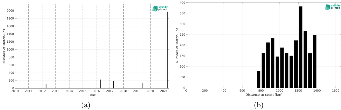
Figure 1: Number of match-ups between TSG (Polarstern) and CCI SSS L4 Merged-OI v4.4 - 30-day running (ESA) SSS as a function of time (a) and as function of the distance to coast (b) over the Amazon and Orinoco river plumes Pi-MEP region and for the full satellite product period.
