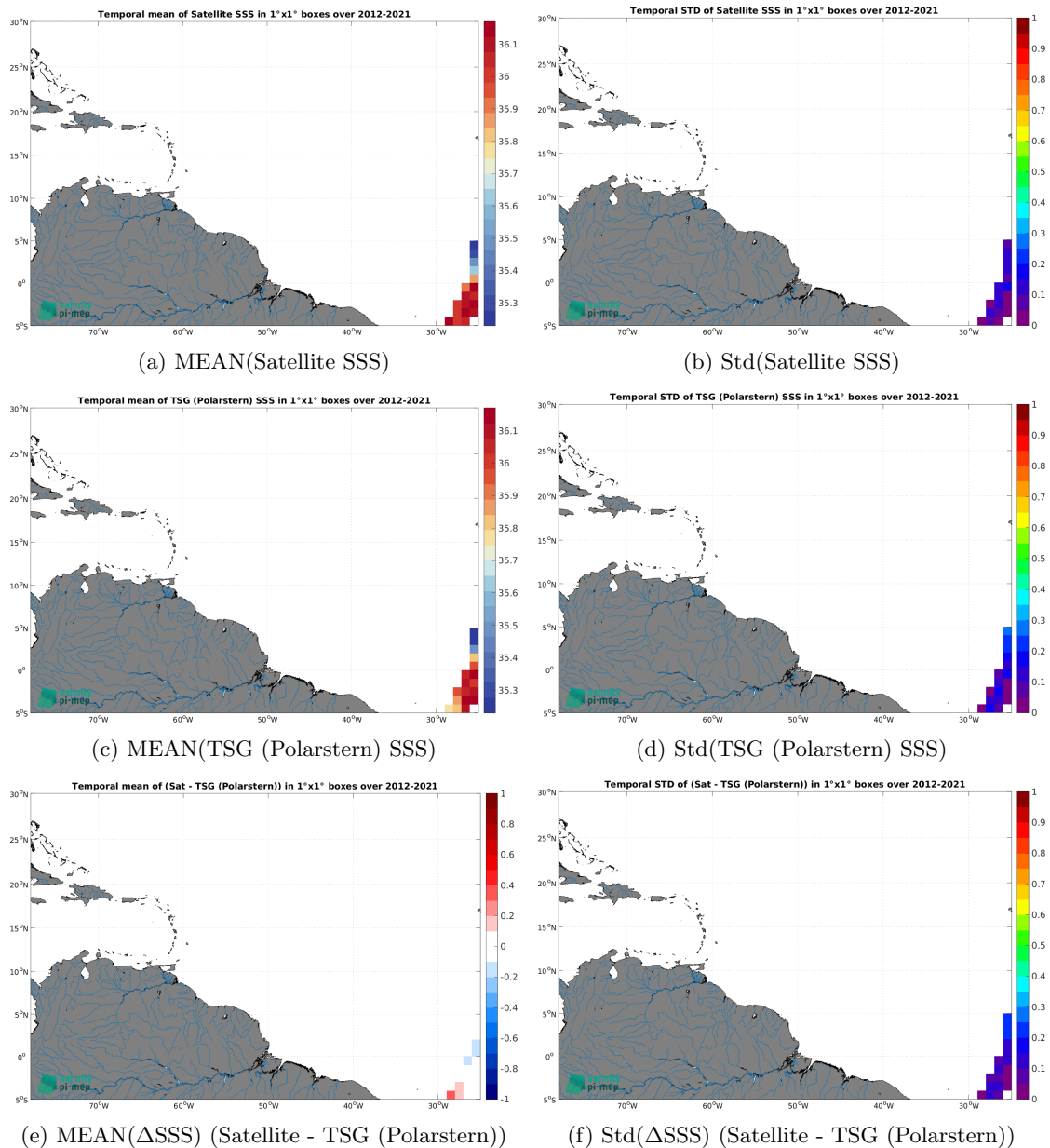
Figure 6: Temporal mean (left) and Std (right) of SSS from CCI SSS L4 Merged-OI v4.4 - 30-day running (ESA) (top), TSG (Polarstern) (middle), and of \Delta SSS (Satellite - TSG (Polarstern)). Only match-up pairs are used to generate these maps.
