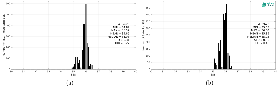
Figure 2: Histograms of SSS from TSG (Polarstern) (a) and CCI SSS L4 Merged-OI v4.4 - 30-day running (ESA) (b) considering all match-up pairs per bins of 0.1 over the Amazon and Orinoco river plumes Pi-MEP region and for the full satellite product period.
