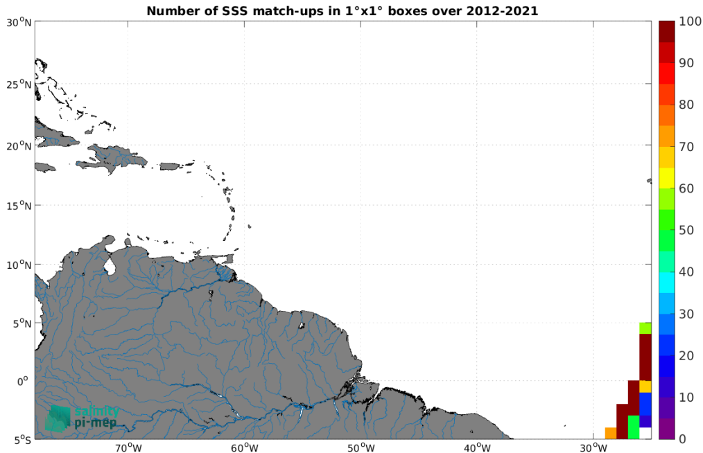
Figure 4: Number of SSS match-ups between TSG (Polarstern) SSS and the CCI SSS L4 Merged-OI v4.4 - 30-day running (ESA) SSS product for the Amazon and Orinoco river plumes Pi-MEP region over 1^\circ \times 1^\circ boxes and for the full satellite product period.
