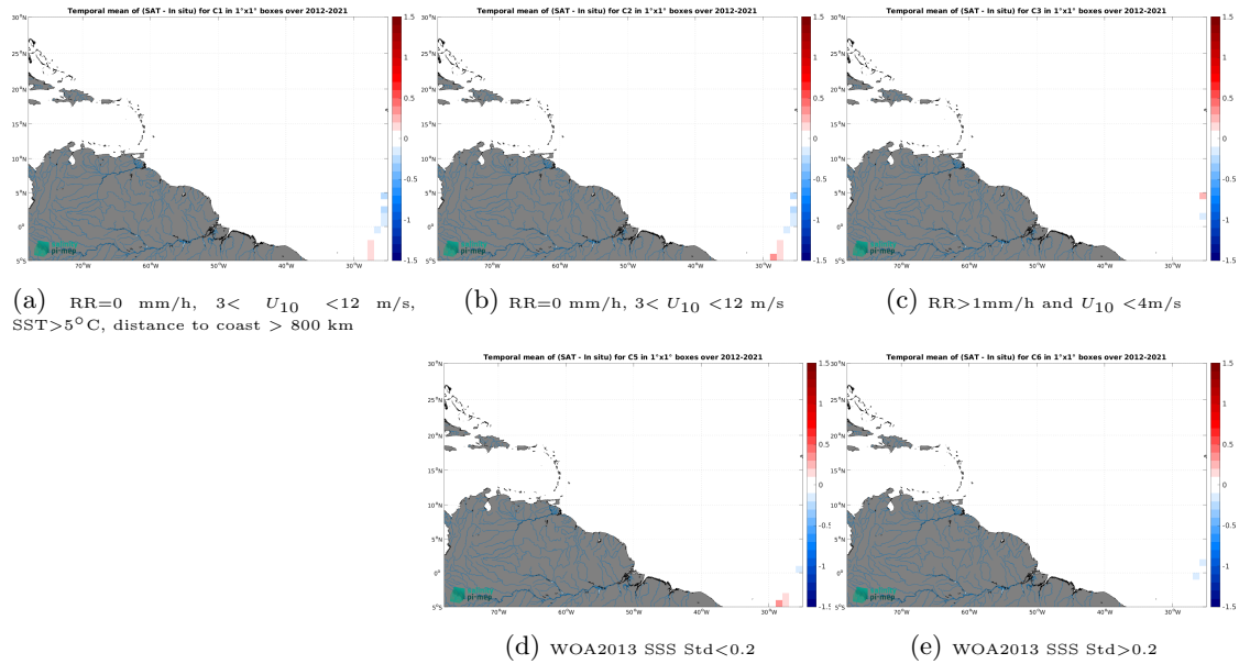
Figure 12: Temporal mean gridded over spatial boxes of size 1^\circ \times 1^\circ of \Delta SSS (CCI SSS L4 Merged-OI v4.4 - 30-day running (ESA) - TSG (Polarstern)) for 5 different subdatasets corresponding to:RR=0 mm/h, 3 < U_{10} < 12 m/s, SST >5^\circ\text{C} , distance to coast > 800 km (a), RR=0 mm/h, 3 < U_{10} < 12 m/s (b), RR >1 mm/h and U_{10} < 4 m/s (c), WOA2013 SSS Std <0.2 (d), WOA2013 SSS Std >0.2 (e).
