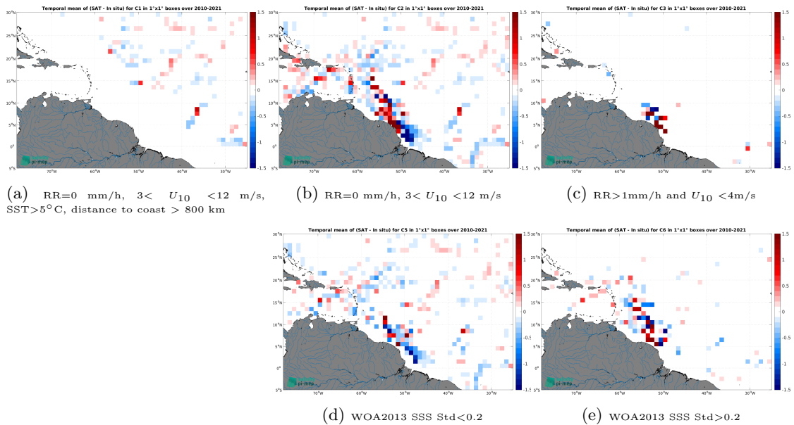
Figure 12: Temporal mean gridded over spatial boxes of size 1^{\circ}\times 1^{\circ} of \Delta SSS (CCI SSS L4 Merged-OI v4.4 - 30-day running (ESA) - TSG (GOSUD-Research-vessel)) for 5 different subdatasets corresponding to:RR=0 mm/h, 3 < U_{10} < 12 m/s, SST >5^{\circ}\text{C} , distance to coast > 800 km (a), RR=0 mm/h, 3 < U_{10} < 12 m/s (b), RR >1 mm/h and U_{10} < 4 m/s (c), WOA2013 SSS Std <0.2 (d), WOA2013 SSS Std >0.2 (e).
