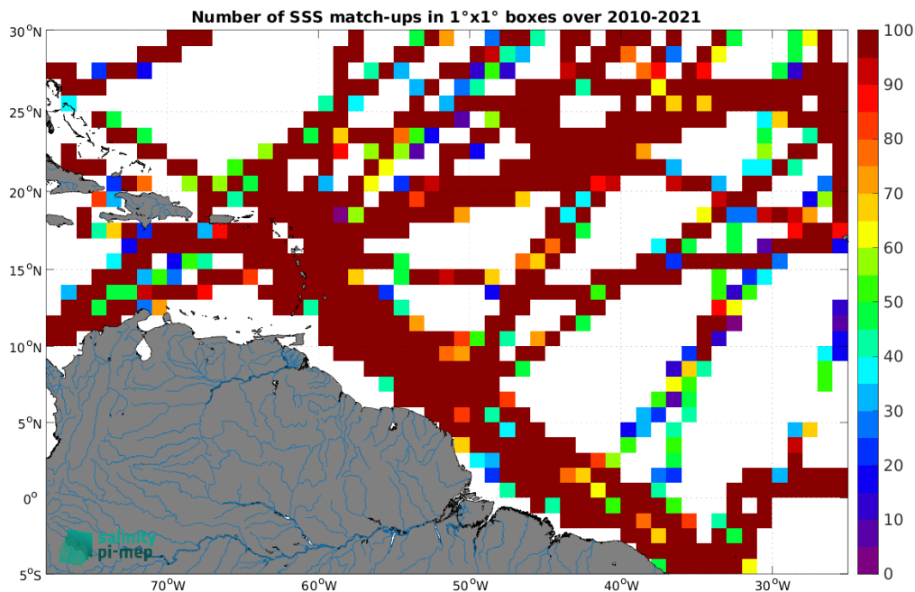
Figure 4: Number of SSS match-ups between TSG (GOSUD-Research-vessel) SSS and the CCI SSS L4 Merged-OI v4.4 - 30-day running (ESA) SSS product for the Amazon and Orinoco river plumes Pi-MEP region over 1^\circ \times 1^\circ boxes and for the full satellite product period.
