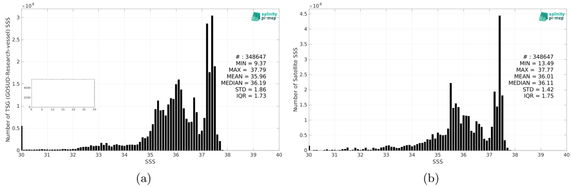
Figure 2: Histograms of SSS from TSG (GOSUD-Research-vessel) (a) and CCI SSS L4 Merged-OI v4.4 - 30-day running (ESA) (b) considering all match-up pairs per bins of 0.1 over the Amazon and Orinoco river plumes Pi-MEP region and for the full satellite product period.
