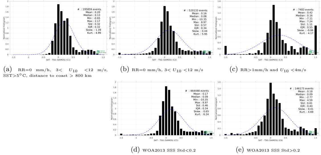
Figure 13: Normalized histogram of \Delta SSS (CCI SSS L4 Merged-OI v3.2 - 7-day running (ESA) - TSG (SAMOS)) for 5 different subdatasets corresponding to: RR=0 mm/h, 3 < U_{10} < 12 m/s, SST > 5°C, distance to coast > 800 km (a), RR=0 mm/h, 3 < U_{10} < 12 m/s (b), RR > 1mm/h and U_{10} < 4 m/s (c), WOA2013 SSS Std < 0.2 (d), WOA2013 SSS Std > 0.2 (e).
