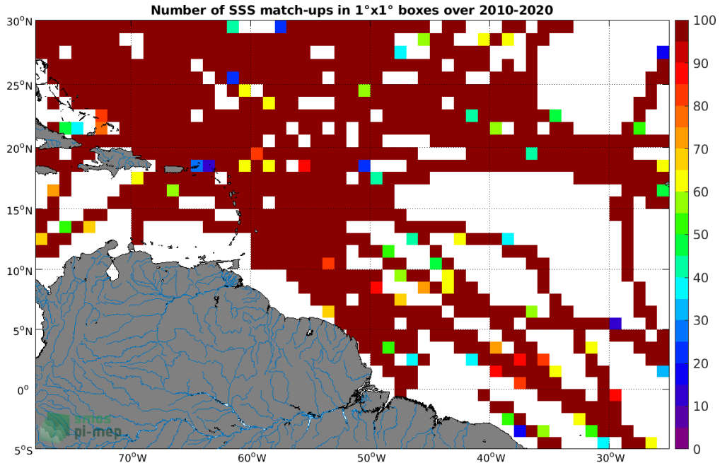
Figure 4: Number of SSS match-ups between TSG (SAMOS) SSS and the CCI SSS L4 Merged-OI v3.2 - 7-day running (ESA) SSS product for the Amazon and Orinoco river plumes Pi-MEP region over 1°x1° boxes and for the full satellite product period.
