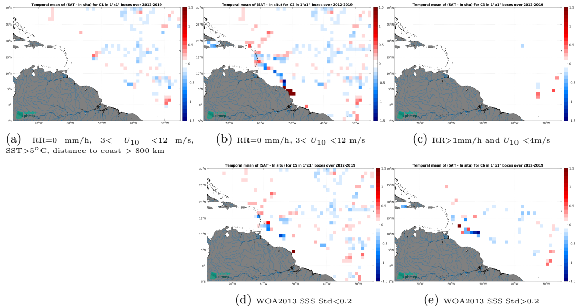
Figure 12: Temporal mean gridded over spatial boxes of size 1^{\circ}\times 1^{\circ} of \Delta SSS (CCI SSS L4 Merged-OI v3.2 - 7-day running (ESA) - TSG (GOSUD-Sailing-ship)) for 5 different subdatasets corresponding to:RR=0 mm/h, 3 < U_{10} < 12 m/s, SST > 5^{\circ}\text{C} , distance to coast > 800 km (a), RR=0 mm/h, 3 < U_{10} < 12 m/s (b), RR > 1 mm/h and U_{10} < 4 m/s (c), WOA2013 SSS Std < 0.2 (d), WOA2013 SSS Std > 0.2 (e).
