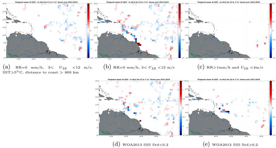
Figure 12: Temporal mean gridded over spatial boxes of size 1^{\circ}\times 1^{\circ} of \Delta SSS (CCI SSS L4 Merged-OI v3.2 - 7-day running (ESA) - TSG (GOSUD-Sailing-ship)) for 5 different subdatasets corresponding to:RR=0 mm/h, 3 < U_{10} < 12 m/s, SST >5^{\circ}\text{C} , distance to coast > 800 km (a), RR=0 mm/h, 3 < U_{10} < 12 m/s (b), RR >1 mm/h and U_{10} < 4 m/s (c), WOA2013 SSS Std <0.2 (d), WOA2013 SSS Std >0.2 (e).
