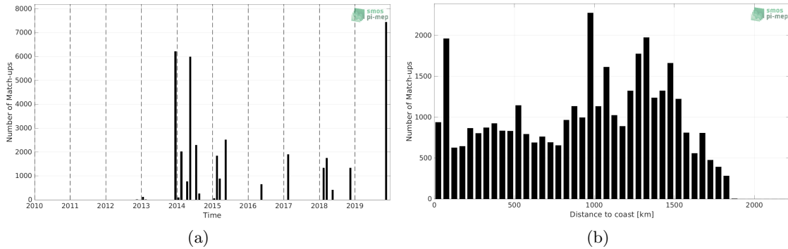
Figure 1: Number of match-ups between TSG (GOSUD-Sailing-ship) and CCI SSS L4 Merged-OI v3.2 - 7-day running (ESA) SSS as a function of time (a) and as function of the distance to coast (b) over the Amazon and Orinoco river plumes Pi-MEP region and for the full satellite product period.
