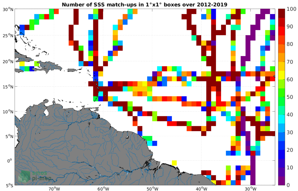
Figure 4: Number of SSS match-ups between TSG (GOSUD-Sailing-ship) SSS and the CCI SSS L4 Merged-OI v3.2 - 7-day running (ESA) SSS product for the Amazon and Orinoco river plumes Pi-MEP region over 1^\circ \times 1^\circ boxes and for the full satellite product period.
