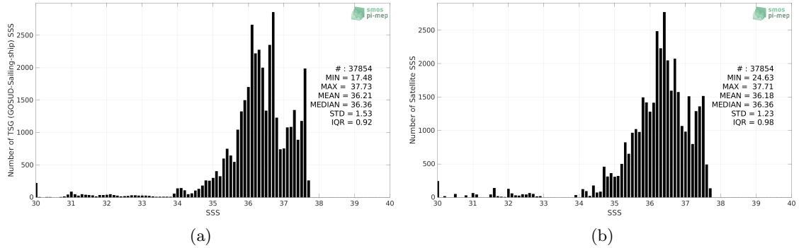
Figure 2: Histograms of SSS from TSG (GOSUD-Sailing-ship) (a) and CCI SSS L4 Merged-OI v3.2 - 7-day running (ESA) (b) considering all match-up pairs per bins of 0.1 over the Amazon and Orinoco river plumes Pi-MEP region and for the full satellite product period.
