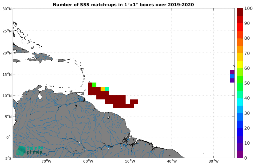
Figure 4: Number of SSS match-ups between Saildrone SSS and the CCI SSS L4 Merged-OI v3.2 - 7-day running (ESA) SSS product for the Amazon and Orinoco river plumes Pi-MEP region over 1^\circ \times 1^\circ boxes and for the full satellite product period.
