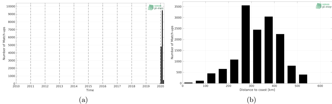
Figure 1: Number of match-ups between Saildrone and CCI SSS L4 Merged-OI v3.2 - 7-day running (ESA) SSS as a function of time (a) and as function of the distance to coast (b) over the Amazon and Orinoco river plumes Pi-MEP region and for the full satellite product period.
