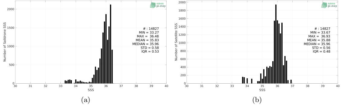
Figure 2: Histograms of SSS from Saildrone (a) and CCI SSS L4 Merged-OI v3.2 - 7-day running (ESA) (b) considering all match-up pairs per bins of 0.1 over the Amazon and Orinoco river plumes Pi-MEP region and for the full satellite product period.
