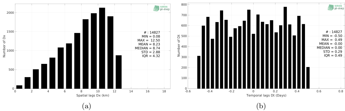
Figure 5: Histograms of the spatial (a) and temporal (b) lags between the location/time of the Sailldrone measurement and the date of the corresponding CCI SSS L4 Merged-OI v3.2 - 7-day running (ESA) SSS pixel.
