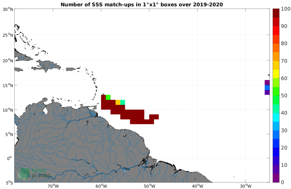
Figure 4: Number of SSS match-ups between Sailldrone SSS and the CCI SSS L4 Merged-OI v3.2 - 7-day running (ESA) SSS product for the Amazon and Orinoco river plumes Pi-MEP region over 1°×1° boxes and for the full satellite product period.
