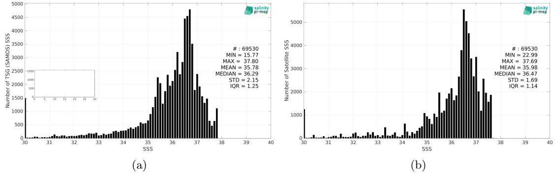
Figure 2: Histograms of SSS from TSG (SAMOS) (a) and CCI SSS L4 Merged-OI v3.2 - 30-day running (ESA) (b) considering all match-up pairs per bins of 0.1 over the Amazon and Orinoco river plumes Pi-MEP region and for the full satellite product period.
