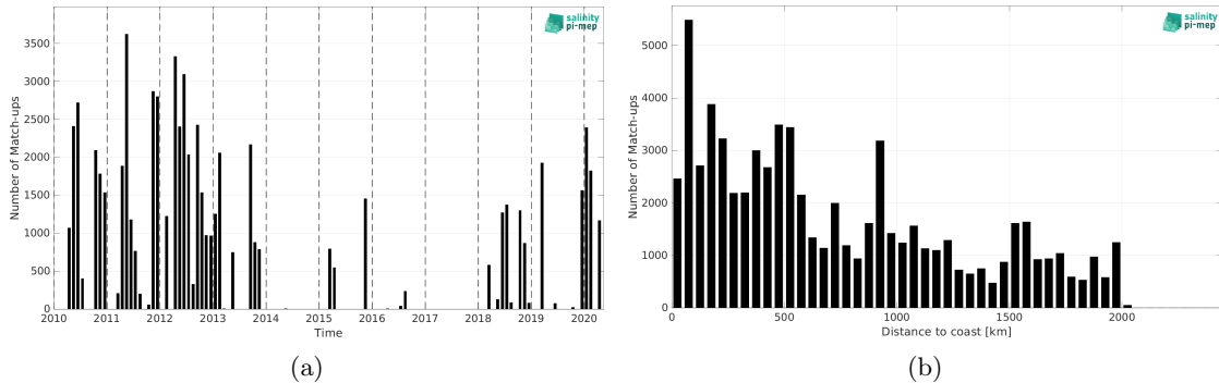
Figure 1: Number of match-ups between TSG (SAMOS) and CCI SSS L4 Merged-OI v3.2 - 30-day running (ESA) SSS as a function of time (a) and as function of the distance to coast (b) over the Amazon and Orinoco river plumes Pi-MEP region and for the full satellite product period.
