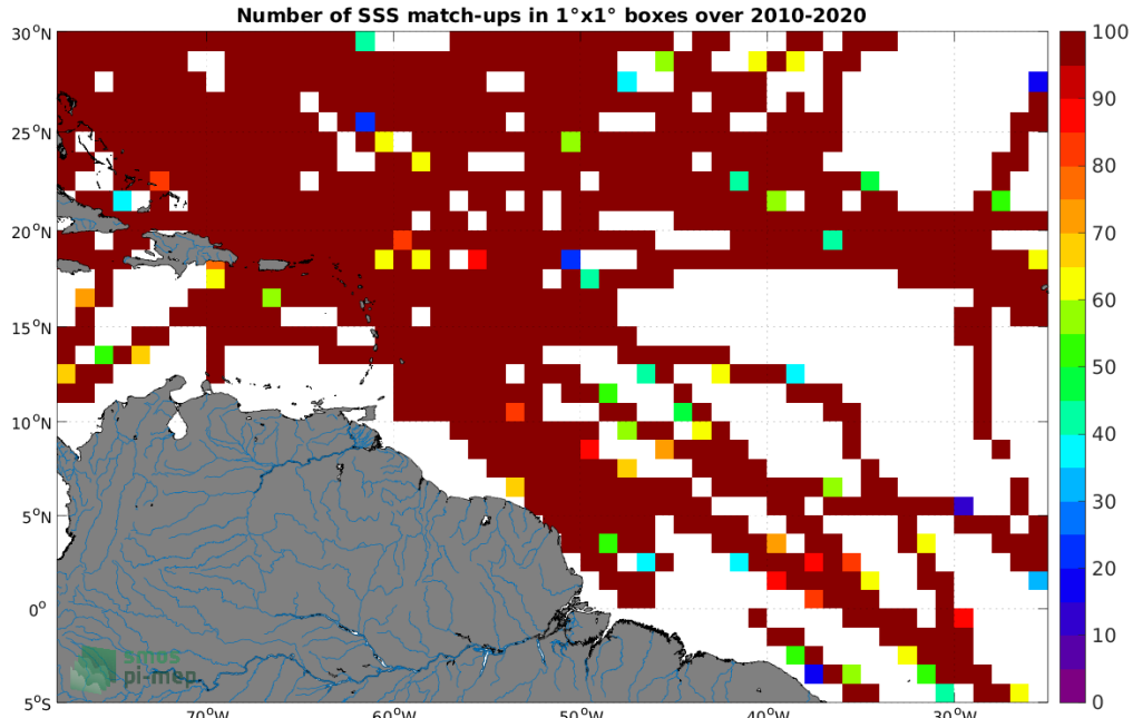
Figure 4: Number of SSS match-ups between TSG (SAMOS) SSS and the CCI SSS L4 Merged-OI v3.2 - 30-day running (ESA) SSS product for the Amazon and Orinoco river plumes Pi-MEP region over 1^\circ \times 1^\circ boxes and for the full satellite product period.
