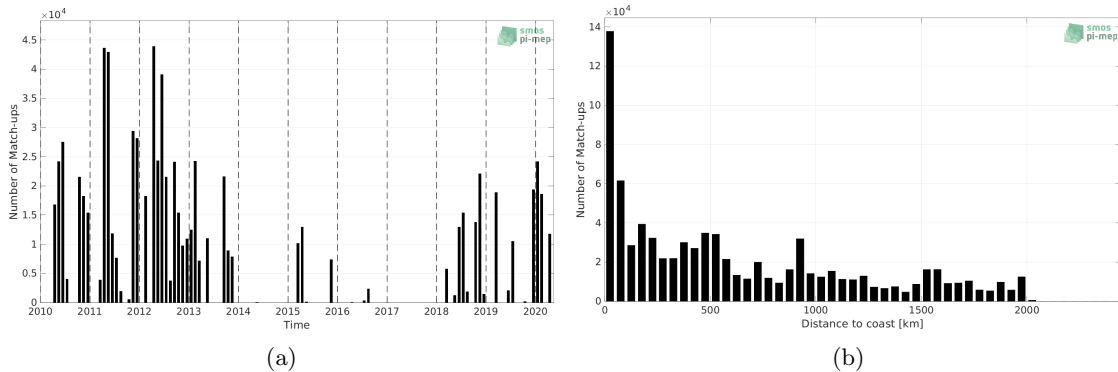
Figure 1: Number of match-ups between TSG (SAMOS) and CCI SSS L4 Merged-OI v3.2 - 30-day running (ESA) SSS as a function of time (a) and as function of the distance to coast (b) over the Amazon and Orinoco river plumes Pi-MEP region and for the full satellite product period.
