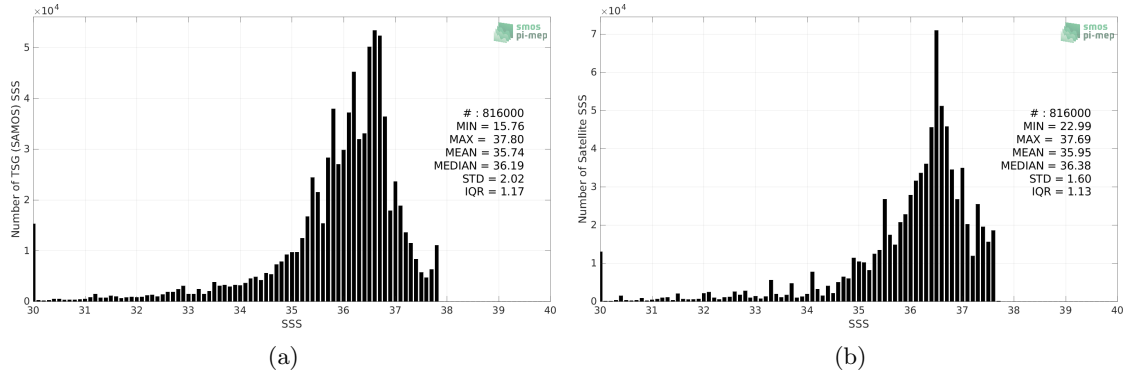
Figure 2: Histograms of SSS from TSG (SAMOS) (a) and CCI SSS L4 Merged-OI v3.2 - 30-day running (ESA) (b) considering all match-up pairs per bins of 0.1 over the Amazon and Orinoco river plumes Pi-MEP region and for the full satellite product period.
