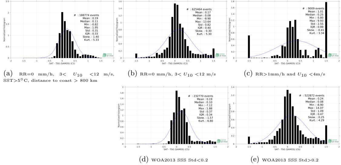
Figure 13: Normalized histogram of \Delta SSS (CCI SSS L4 Merged-OI v3.2 - 30-day running (ESA) - TSG (SAMOS)) for 5 different subdatasets corresponding to: RR=0 mm/h, 3 < U_{10} < 12 m/s, SST>5°C, distance to coast > 800 km (a), RR=0 mm/h, 3 < U_{10} < 12 m/s (b), RR>1mm/h and U_{10} < 4 m/s (c), WOA2013 SSS Std<0.2 (d), WOA2013 SSS Std>0.2 (e).
