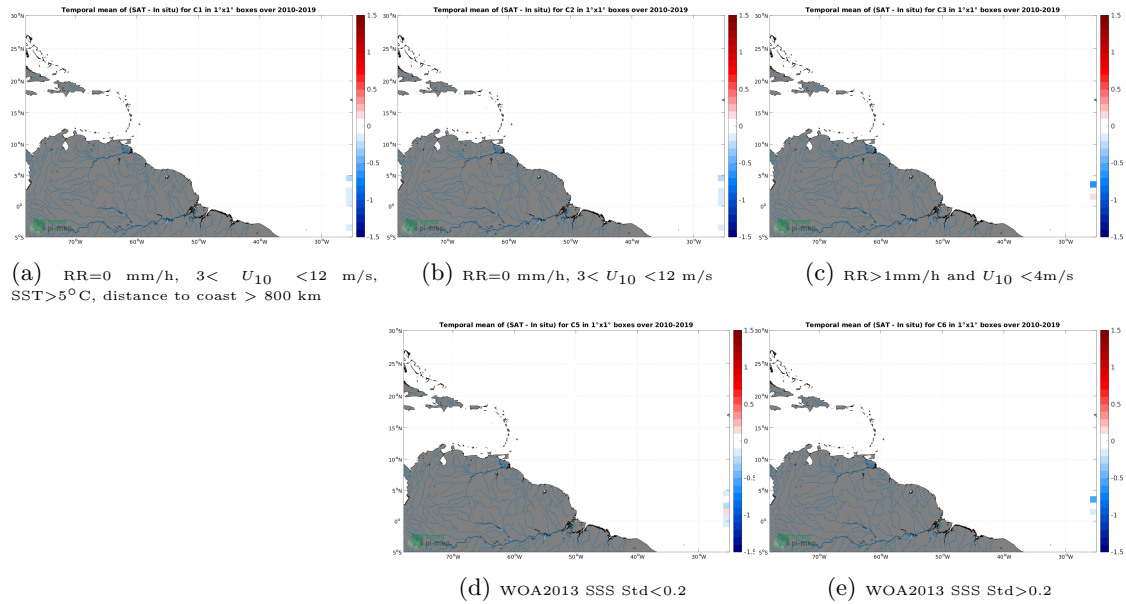
Figure 12: Temporal mean gridded over spatial boxes of size 1^\circ \times 1^\circ of \Delta SSS (CCI SSS L4 Merged-OI v3.2 - 30-day running (ESA) - TSG (Polarstern)) for 5 different subdatasets corresponding to:RR=0 mm/h, 3 < U_{10} < 12 m/s, SST >5^\circ C, distance to coast > 800 km (a), RR=0 mm/h, 3 < U_{10} < 12 m/s (b), RR >1 mm/h and U_{10} < 4 m/s (c), WOA2013 SSS Std <0.2 (d), WOA2013 SSS Std >0.2 (e).
