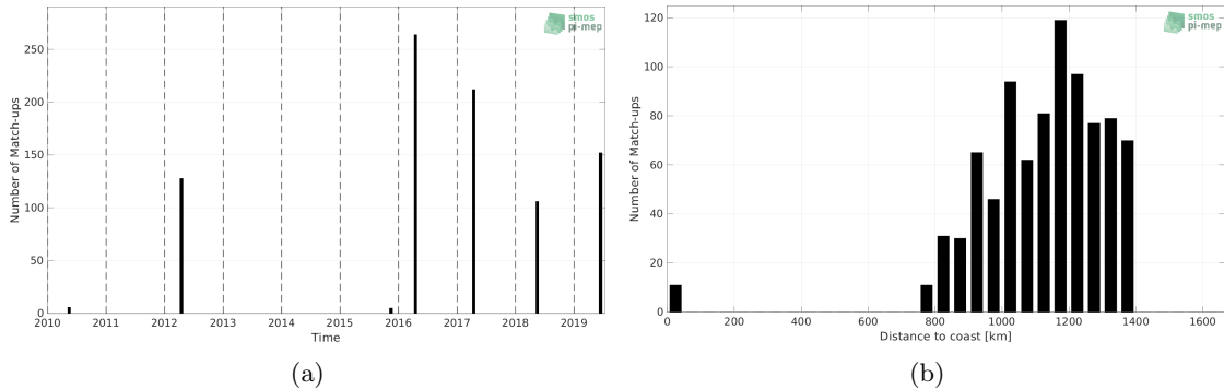
Figure 1: Number of match-ups between TSG (Polarstern) and CCI SSS L4 Merged-OI v3.2 - 30-day running (ESA) SSS as a function of time (a) and as function of the distance to coast (b) over the Amazon and Orinoco river plumes Pi-MEP region and for the full satellite product period.
