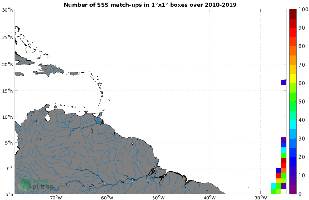
Figure 4: Number of SSS match-ups between TSG (Polarstern) SSS and the CCI SSS L4 Merged-OI v3.2 - 30-day running (ESA) SSS product for the Amazon and Orinoco river plumes Pi-MEP region over 1^\circ \times 1^\circ boxes and for the full satellite product period.
