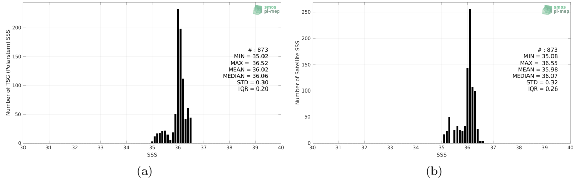
Figure 2: Histograms of SSS from TSG (Polarstern) (a) and CCI SSS L4 Merged-OI v3.2 - 30-day running (ESA) (b) considering all match-up pairs per bins of 0.1 over the Amazon and Orinoco river plumes Pi-MEP region and for the full satellite product period.
