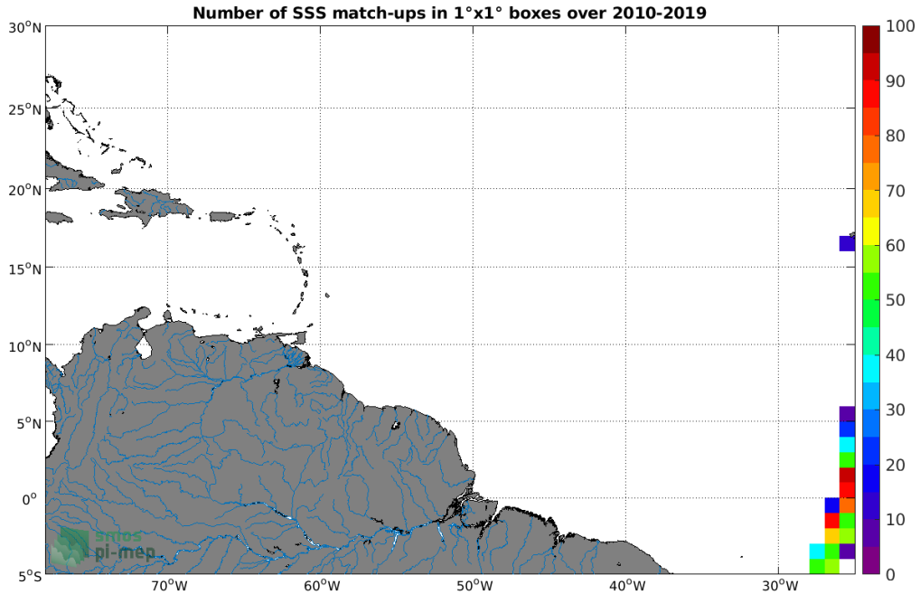
Figure 4: Number of SSS match-ups between TSG (Polarstern) SSS and the CCI SSS L4 Merged-OI v3.2 - 30-day running (ESA) SSS product for the Amazon and Orinoco river plumes Pi-MEP region over 1°x1° boxes and for the full satellite product period.
