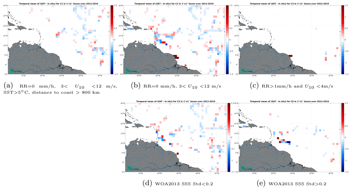
Figure 12: Temporal mean gridded over spatial boxes of size 1^{\circ}\times 1^{\circ} of \Delta SSS (CCI SSS L4 Merged-OI v3.2 - 30-day running (ESA) - TSG (GOSUD-Sailing-ship)) for 5 different subdatasets corresponding to:RR=0 mm/h, 3 < U_{10} < 12 m/s, SST >5^{\circ}\text{C} , distance to coast > 800 km (a), RR=0 mm/h, 3 < U_{10} < 12 m/s (b), RR >1 mm/h and U_{10} < 4 m/s (c), WOA2013 SSS Std <0.2 (d), WOA2013 SSS Std >0.2 (e).
