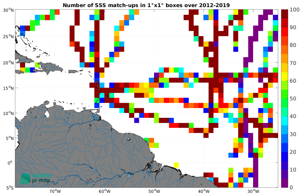
Figure 4: Number of SSS match-ups between TSG (GOSUD-Sailing-ship) SSS and the CCI SSS L4 Merged-OI v3.2 - 30-day running (ESA) SSS product for the Amazon and Orinoco river plumes Pi-MEP region over 1^{\circ} \times 1^{\circ} boxes and for the full satellite product period.
