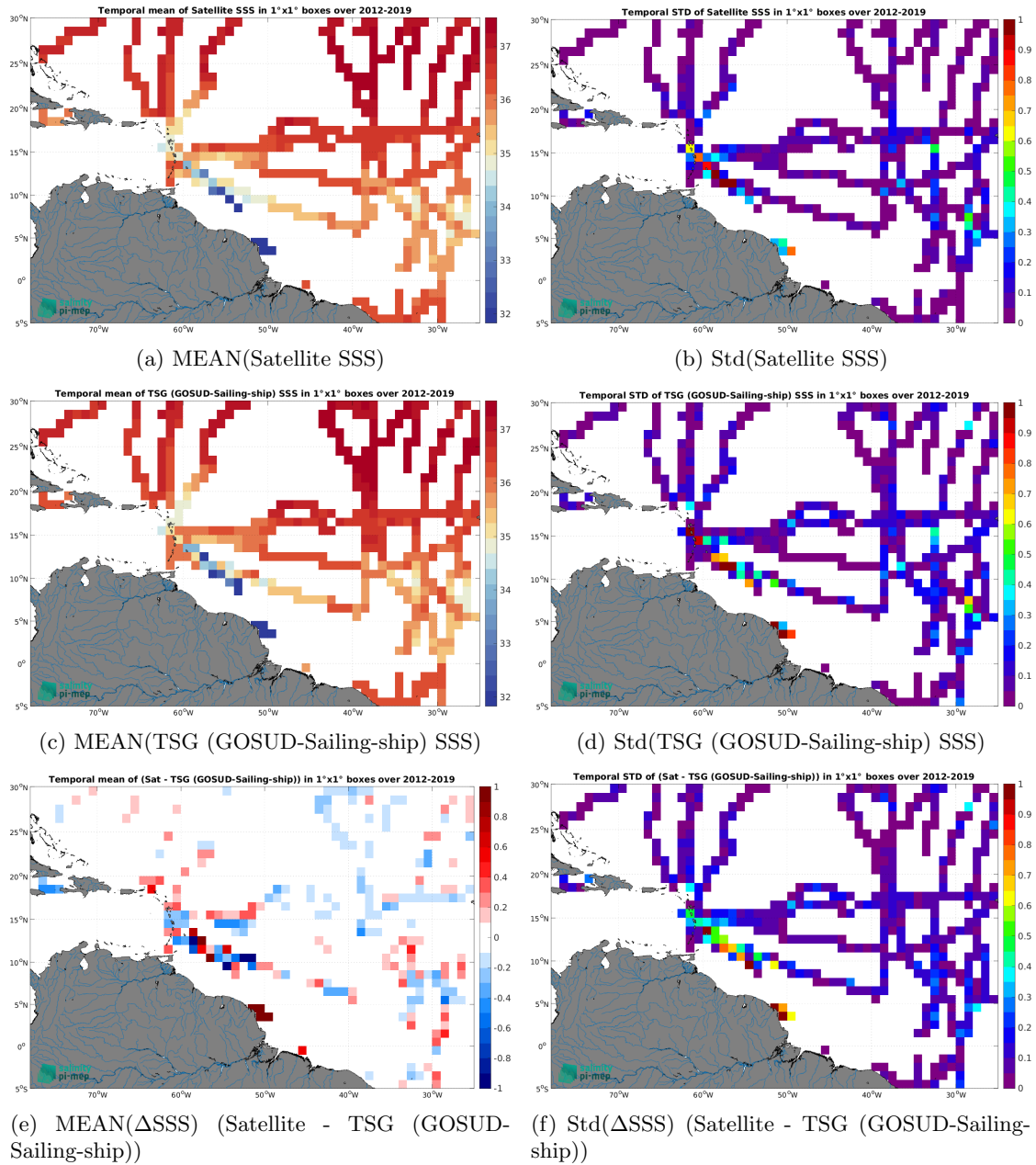
Figure 6: Temporal mean (left) and Std (right) of SSS from CCI SSS L4 Merged-OI v3.2 - 30-day running (ESA) (top), TSG (GOSUD-Sailing-ship) (middle), and of \Delta SSS (Satellite - TSG (GOSUD-Sailing-ship)). Only match-up pairs are used to generate these maps.
