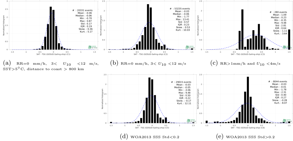
Figure 13: Normalized histogram of \Delta SSS (CCI SSS L4 Merged-OI v3.2 - 30-day running (ESA) - TSG (GOSUD-Sailing-ship)) for 5 different subdatasets corresponding to: RR=0 mm/h, 3 < U_{10} < 12 m/s, SST>5°C, distance to coast > 800 km (a), RR=0 mm/h, 3 < U_{10} < 12 m/s (b), RR>1mm/h and U_{10} < 4 m/s (c), WOA2013 SSS Std<0.2 (d), WOA2013 SSS Std>0.2 (e).
