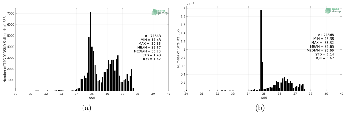
Figure 2: Histograms of SSS from TSG (GOSUD-Sailing-ship) (a) and CCI SSS L4 Merged-OI v3.2 - 30-day running (ESA) (b) considering all match-up pairs per bins of 0.1 over the Amazon and Orinoco river plumes Pi-MEP region and for the full satellite product period.
