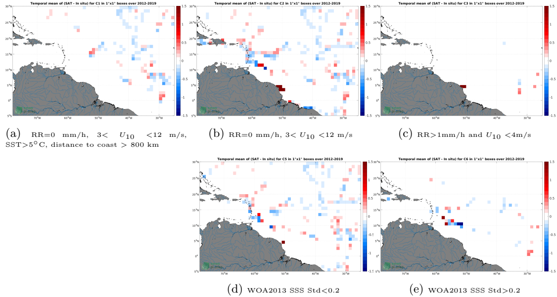
Figure 12: Temporal mean gridded over spatial boxes of size 1^\circ \times 1^\circ of \Delta SSS (CCI SSS L4 Merged-OI v3.2 - 30-day running (ESA) - TSG (GOSUD-Sailing-ship)) for 5 different subdatasets corresponding to:RR=0 mm/h, 3 < U_{10} < 12 m/s, SST >5^\circ\text{C} , distance to coast > 800 km (a), RR=0 mm/h, 3 < U_{10} < 12 m/s (b), RR >1 mm/h and U_{10} < 4 m/s (c), WOA2013 SSS Std <0.2 (d), WOA2013 SSS Std >0.2 (e).
