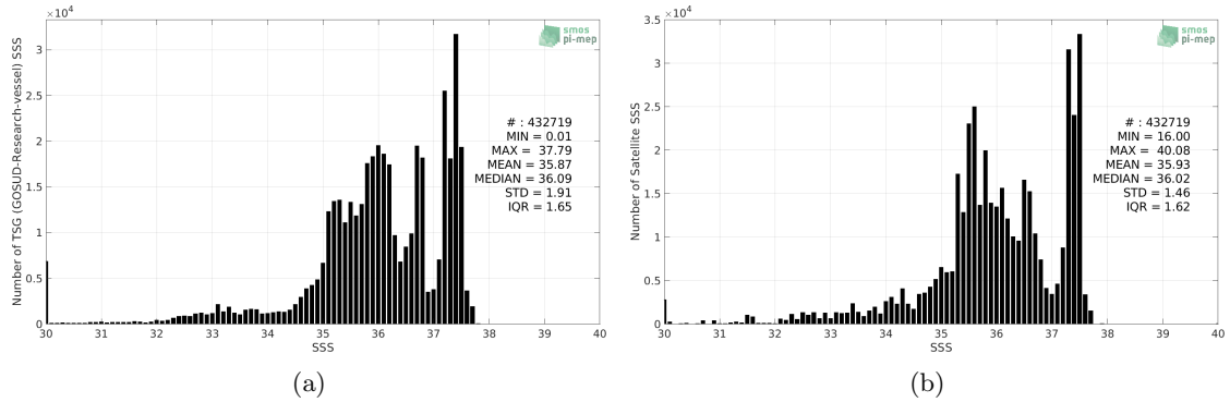
Figure 2: Histograms of SSS from TSG (GOSUD-Research-vessel) (a) and CCI SSS L4 Merged-OI v3.2 - 30-day running (ESA) (b) considering all match-up pairs per bins of 0.1 over the Amazon and Orinoco river plumes Pi-MEP region and for the full satellite product period.
