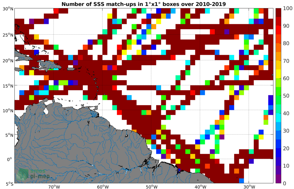
Figure 4: Number of SSS match-ups between TSG (GOSUD-Research-vessel) SSS and the CCI SSS L4 Merged-OI v3.2 - 30-day running (ESA) SSS product for the Amazon and Orinoco river plumes Pi-MEP region over 1^\circ \times 1^\circ boxes and for the full satellite product period.
