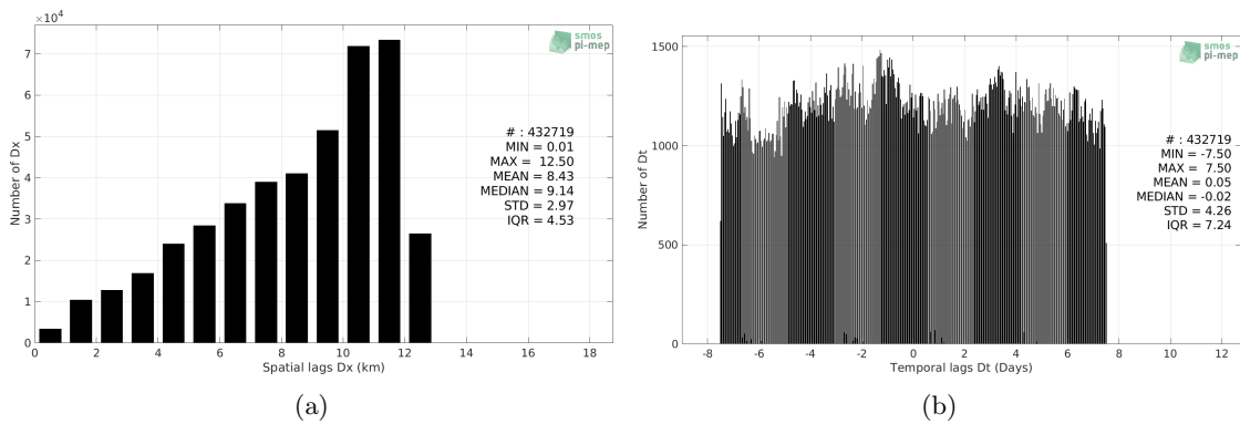
Figure 5: Histograms of the spatial (a) and temporal (b) lags between the location/time of the TSG (GOSUD-Research-vessel) measurement and the date of the corresponding CCI SSS L4 Merged-OI v3.2 - 30-day running (ESA) SSS pixel.
