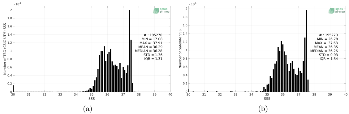
Figure 2: Histograms of SSS from TSG (CSIC-UTM) (a) and CCI SSS L4 Merged-OI v3.2 - 30-day running (ESA) (b) considering all match-up pairs per bins of 0.1 over the Amazon and Orinoco river plumes Pi-MEP region and for the full satellite product period.
