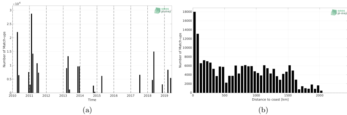
Figure 1: Number of match-ups between TSG (CSIC-UTM) and CCI SSS L4 Merged-OI v3.2 - 30-day running (ESA) SSS as a function of time (a) and as function of the distance to coast (b) over the Amazon and Orinoco river plumes Pi-MEP region and for the full satellite product period.
