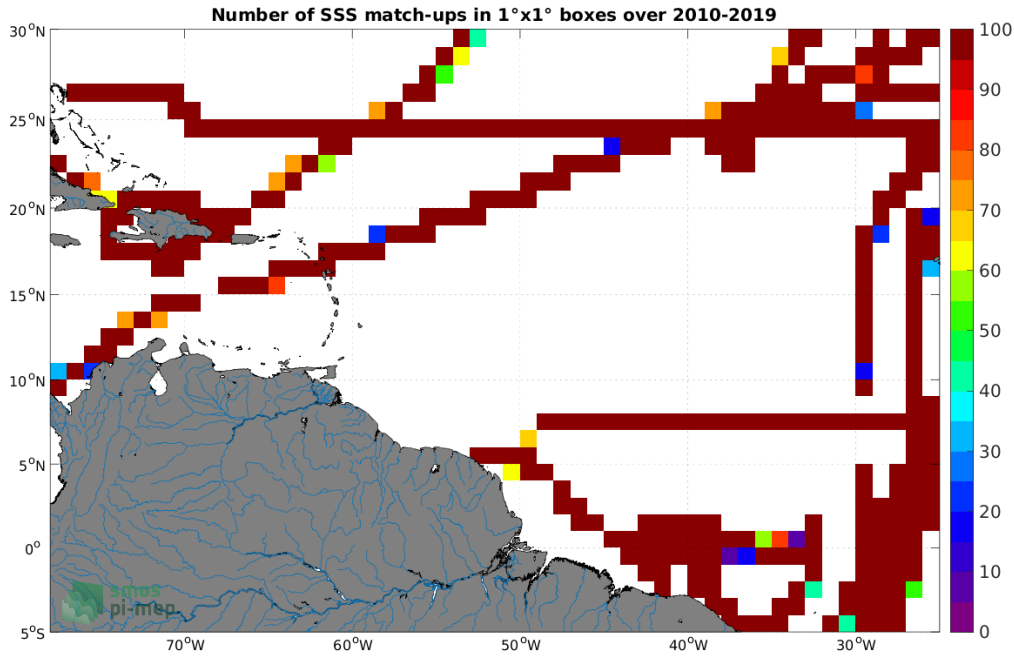
Figure 4: Number of SSS match-ups between TSG (CSIC-UTM) SSS and the CCI SSS L4 Merged-OI v3.2 - 30-day running (ESA) SSS product for the Amazon and Orinoco river plumes Pi-MEP region over 1^\circ \times 1^\circ boxes and for the full satellite product period.
