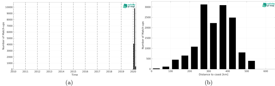
Figure 1: Number of match-ups between Sairdrone and CCI SSS L4 Merged-OI v3.2 - 30-day running (ESA) SSS as a function of time (a) and as function of the distance to coast (b) over the Amazon and Orinoco river plumes Pi-MEP region and for the full satellite product period.
