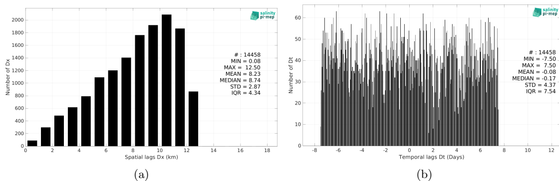
Figure 5: Histograms of the spatial (a) and temporal (b) lags between the location/time of the Sailldrone measurement and the date of the corresponding CCI SSS L4 Merged-OI v3.2 - 30-day running (ESA) SSS pixel.
