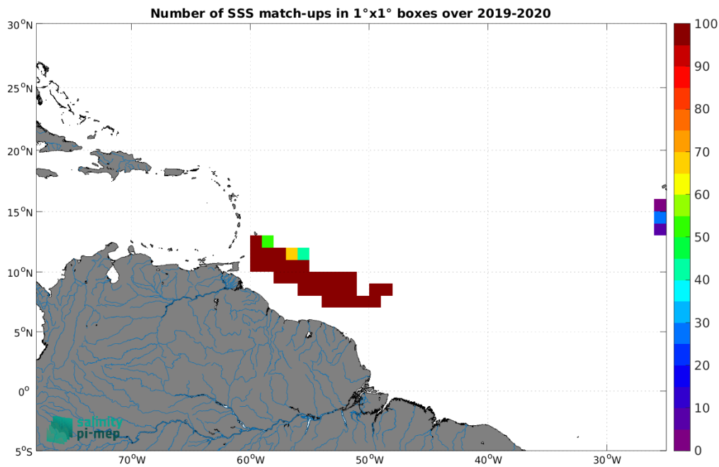
Figure 4: Number of SSS match-ups between Sailldrone SSS and the CCI SSS L4 Merged-OI v3.2 - 30-day running (ESA) SSS product for the Amazon and Orinoco river plumes Pi-MEP region over 1^\circ \times 1^\circ boxes and for the full satellite product period.
