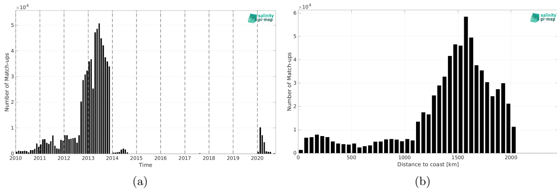
Figure 1: Number of match-ups between Surface drifters and CCI SSS L4 Merged-OI v3.2 - 30-day running (ESA) SSS as a function of time (a) and as function of the distance to coast (b) over the Amazon and Orinoco river plumes Pi-MEP region and for the full satellite product period.
