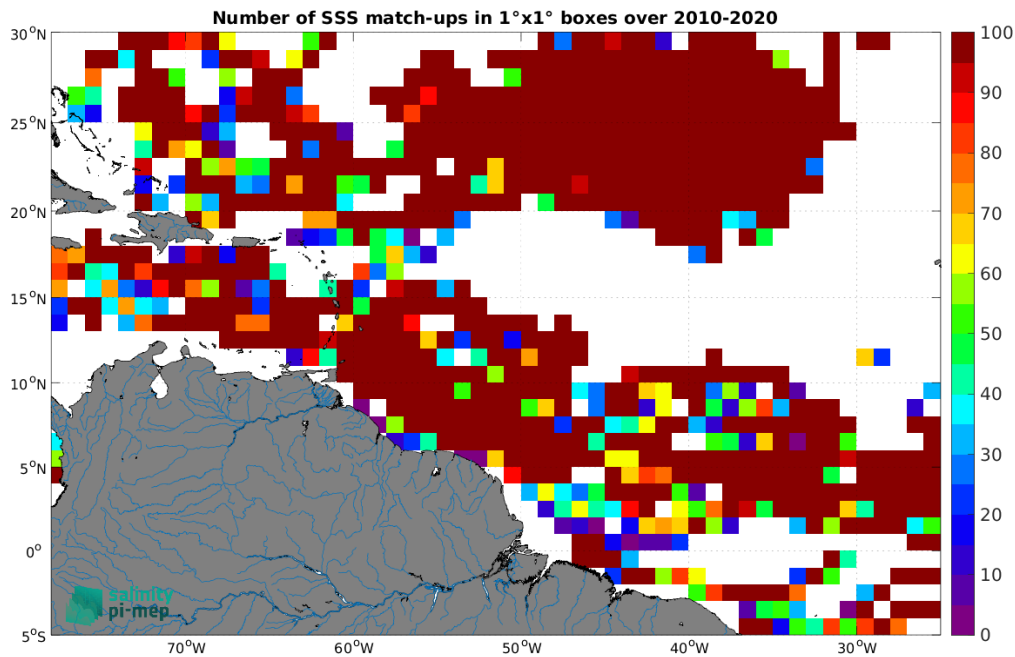
Figure 3: Number of SSS match-ups between Surface drifters SSS and the CCI SSS L4 Merged-OI v3.2 - 30-day running (ESA) SSS product for the Amazon and Orinoco river plumes Pi-MEP region over 1^\circ \times 1^\circ boxes and for the full satellite product period.
