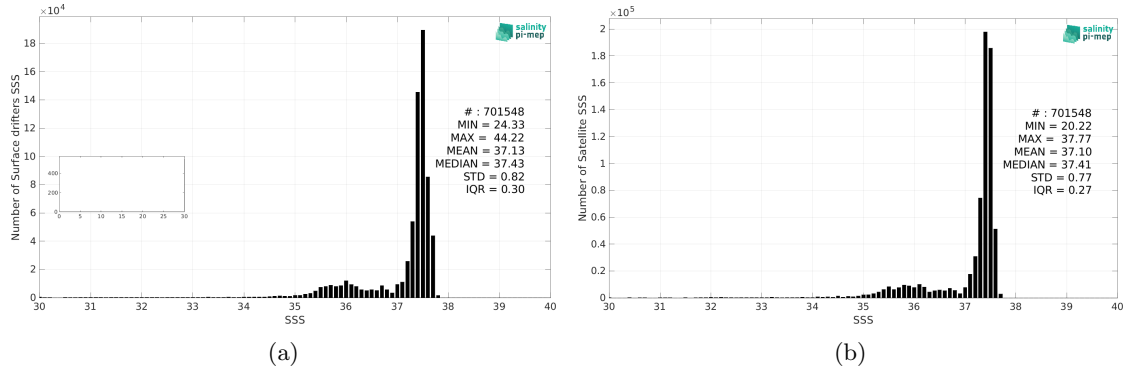
Figure 2: Histograms of SSS from Surface drifters (a) and CCI SSS L4 Merged-OI v3.2 - 30-day running (ESA) (b) considering all match-up pairs per bins of 0.1 over the Amazon and Orinoco river plumes Pi-MEP region and for the full satellite product period.
