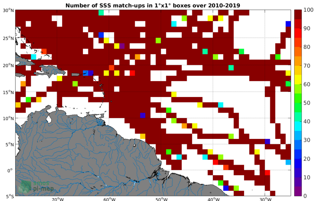
Figure 4: Number of SSS match-ups between TSG (SAMOS) SSS and the CCI SSS L4 Merged-OI v2.31 - 7-day running (ESA) SSS product for the Amazon and Orinoco river plumes Pi-MEP region over 1^\circ \times 1^\circ boxes and for the full satellite product period.
