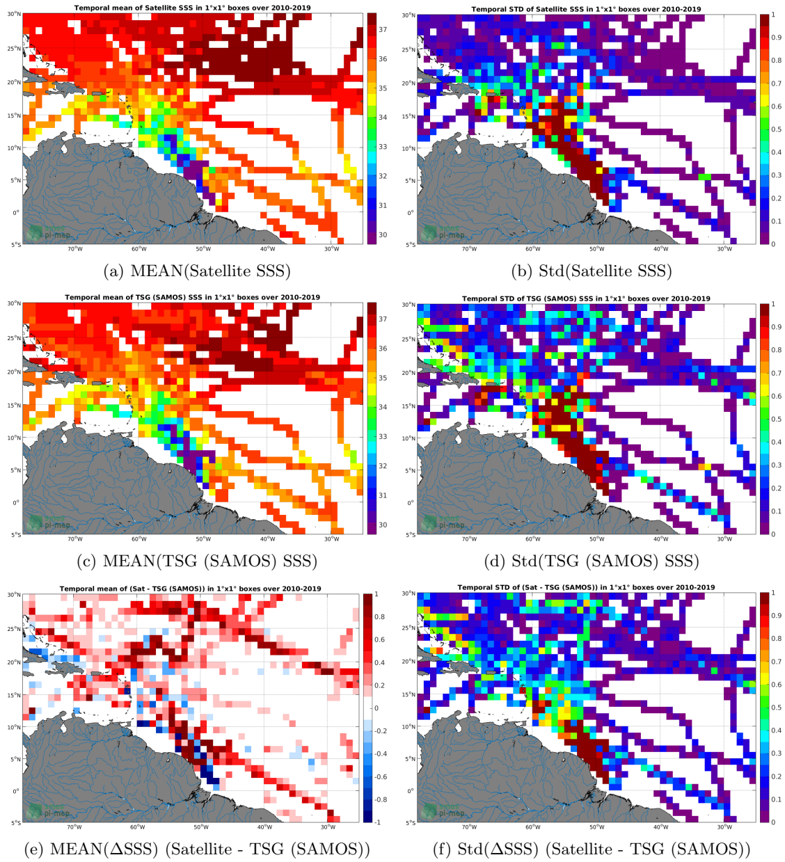
Figure 6: Temporal mean (left) and Std (right) of SSS from CCI SSS L4 Merged-OI v2.31 - 7-day running (ESA) (top), TSG (SAMOS) (middle), and of \Delta SSS (Satellite - TSG (SAMOS)). Only match-up pairs are used to generate these maps.
