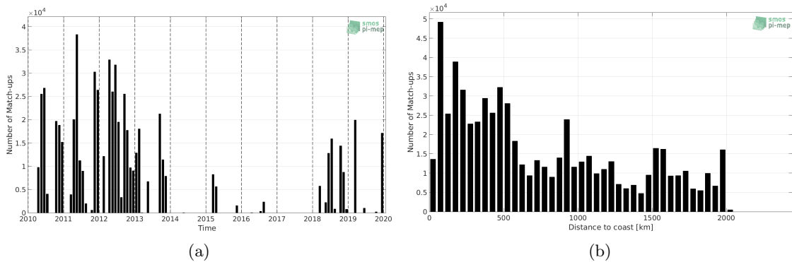
Figure 1: Number of match-ups between TSG (SAMOS) and CCI SSS L4 Merged-OI v2.31 - 7-day running (ESA) SSS as a function of time (a) and as function of the distance to coast (b) over the Amazon and Orinoco river plumes Pi-MEP region and for the full satellite product period.
