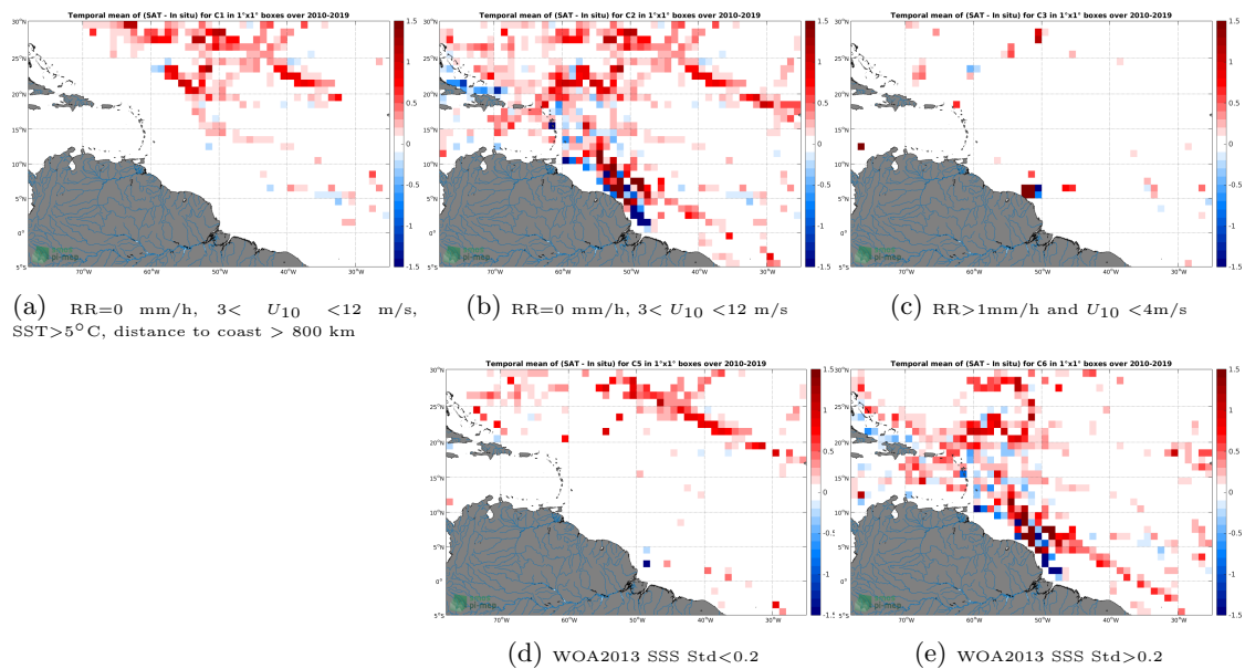
Figure 12: Temporal mean gridded over spatial boxes of size 1^\circ \times 1^\circ of \Delta SSS (CCI SSS L4 Merged-OI v2.31 - 7-day running (ESA) - TSG (SAMOS)) for 5 different subdatasets corresponding to:RR=0 mm/h, 3 < U_{10} < 12 m/s, SST >5^\circ C, distance to coast > 800 km (a), RR=0 mm/h, 3 < U_{10} < 12 m/s (b), RR >1 mm/h and U_{10} < 4 m/s (c), WOA2013 SSS Std <0.2 (d), WOA2013 SSS Std >0.2 (e).
