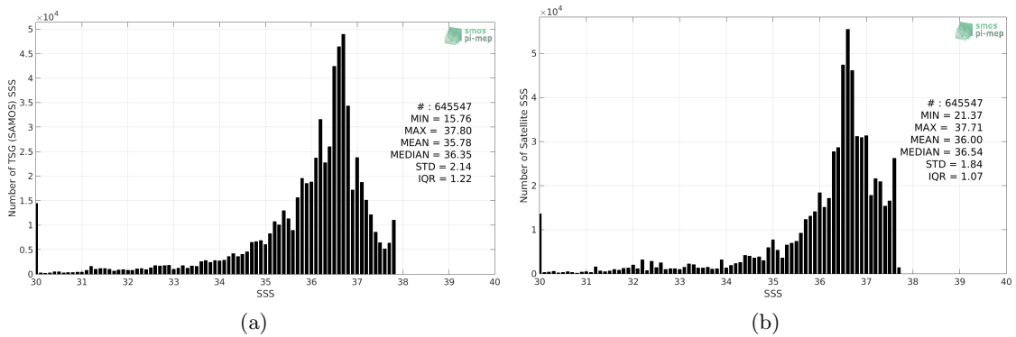
Figure 2: Histograms of SSS from TSG (SAMOS) (a) and CCI SSS L4 Merged-OI v2.31 - 7-day running (ESA) (b) considering all match-up pairs per bins of 0.1 over the Amazon and Orinoco river plumes Pi-MEP region and for the full satellite product period.
