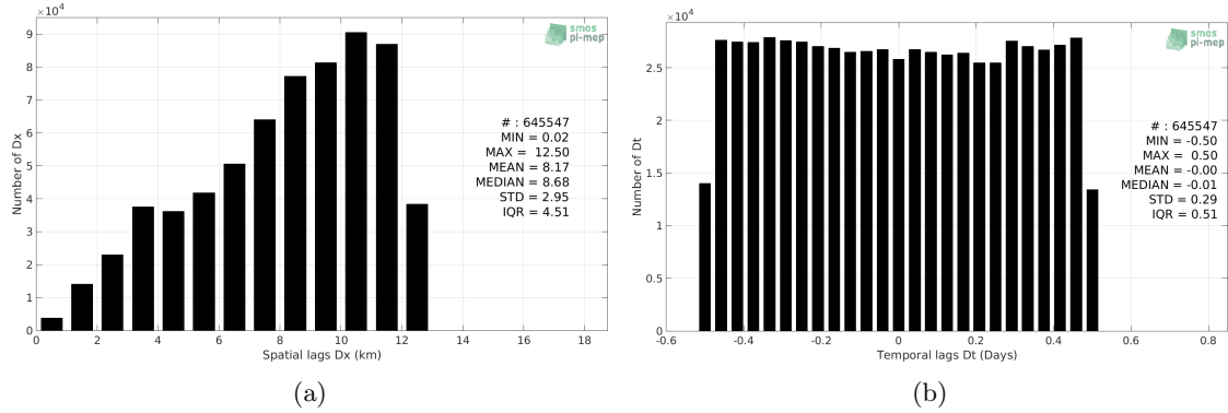
Figure 5: Histograms of the spatial (a) and temporal (b) lags between the time of the TSG (SAMOS) measurements and the date of the corresponding CCI SSS L4 Merged-OI v2.31 - 7-day running (ESA) SSS product.
