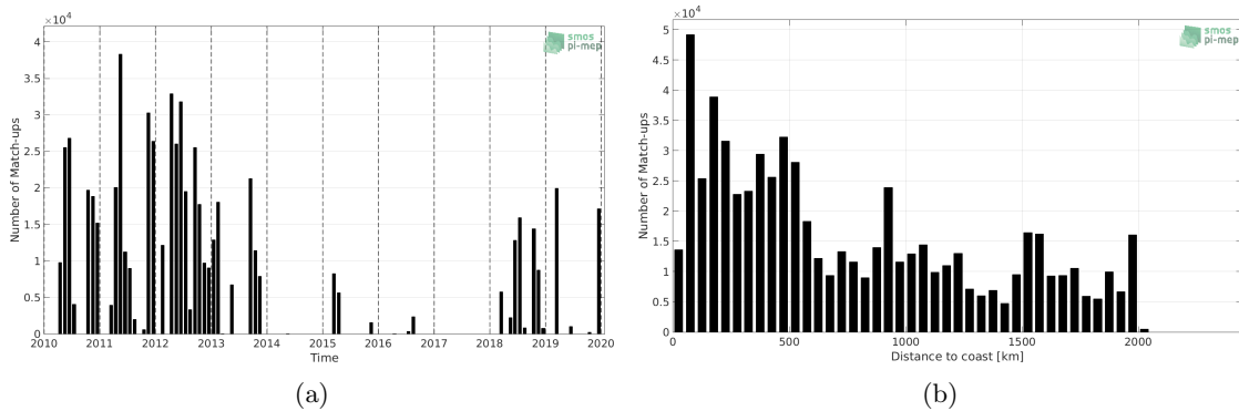
Figure 1: Number of match-ups between TSG (SAMOS) and CCI L4 Merged-OI v2.31 - 7-day running (ESA) SSS as a function of time (a) and as function of the distance to coast (b) over the Amazon and Orinoco river plumes Pi-MEP region and for the full satellite product period.
