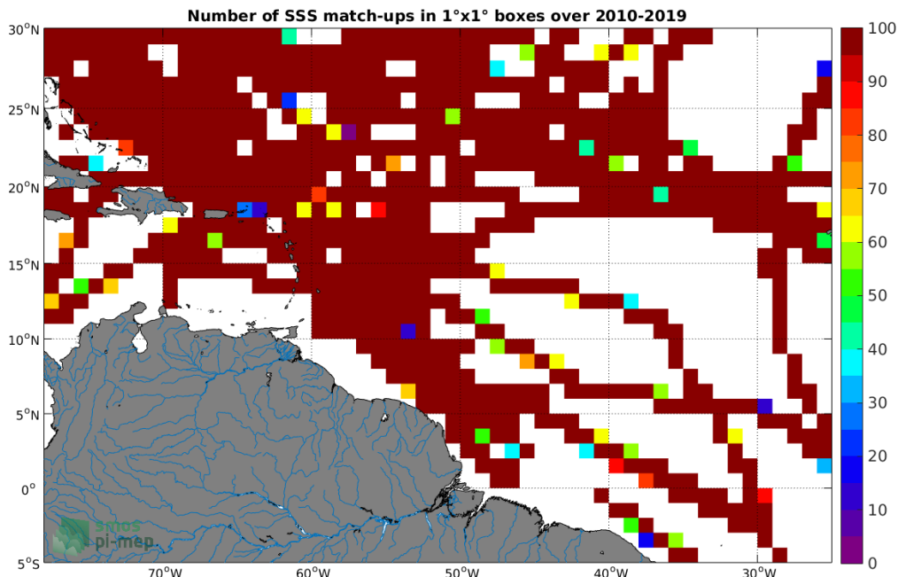
Figure 4: Number of SSS match-ups between TSG (SAMOS) SSS and the CCI L4 Merged-OI v2.31 - 7-day running (ESA) SSS product for the Amazon and Orinoco river plumes Pi-MEP region over 1°x1° boxes and for the full satellite product period.
