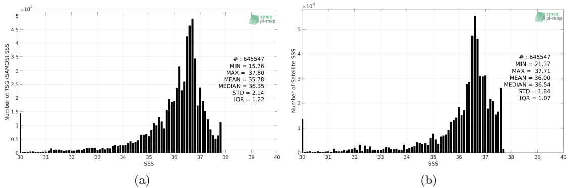
Figure 2: Histograms of SSS from TSG (SAMOS) (a) and CCI L4 Merged-OI v2.31 - 7-day running (ESA) (b) considering all match-up pairs per bins of 0.1 over the Amazon and Orinoco river plumes Pi-MEP region and for the full satellite product period.
