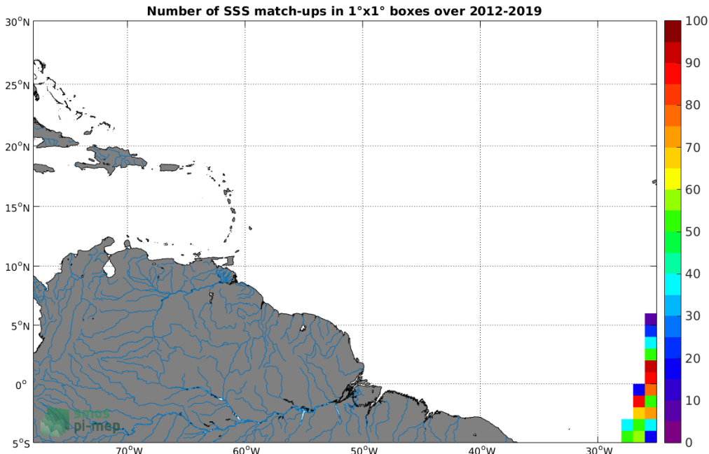
Figure 4: Number of SSS match-ups between TSG (Polarstern) SSS and the CCI SSS L4 Merged-OI v2.31 - 7-day running (ESA) SSS product for the Amazon and Orinoco river plumes Pi-MEP region over 1°x1° boxes and for the full satellite product period.
