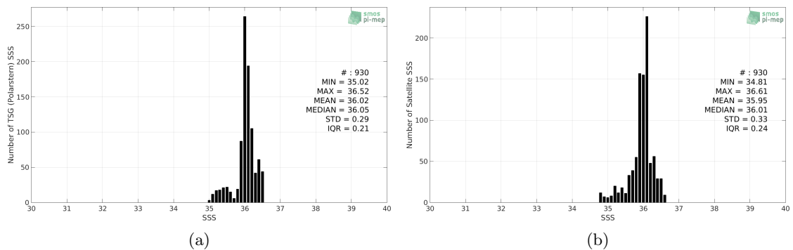
Figure 2: Histograms of SSS from TSG (Polarstern) (a) and CCI SSS L4 Merged-OI v2.31 - 7-day running (ESA) (b) considering all match-up pairs per bins of 0.1 over the Amazon and Orinoco river plumes Pi-MEP region and for the full satellite product period.
