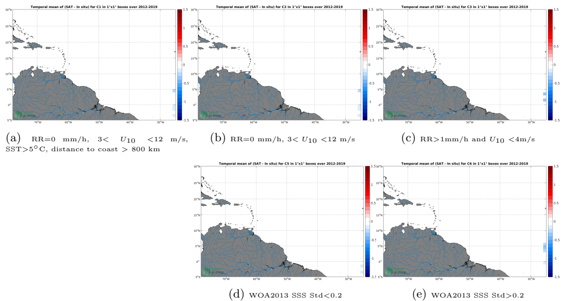
Figure 12: Temporal mean gridded over spatial boxes of size 1^\circ \times 1^\circ of \Delta SSS (CCI L4 Merged-OI v2.31 - 7-day running (ESA) - TSG (Polarstern)) for 5 different subdatasets corresponding to:RR=0 mm/h, 3 < U_{10} < 12 m/s, SST >5^\circ C, distance to coast > 800 km (a), RR=0 mm/h, 3 < U_{10} < 12 m/s (b), RR >1 mm/h and U_{10} < 4 m/s (c), WOA2013 SSS Std <0.2 (d), WOA2013 SSS Std >0.2 (e).
