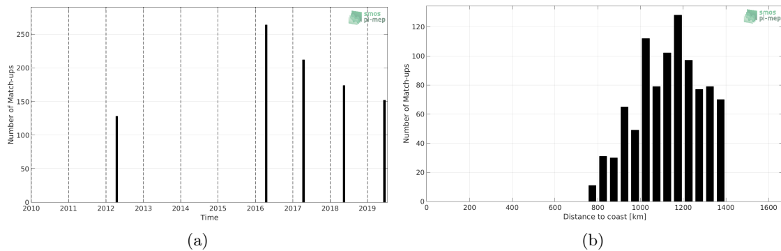
Figure 1: Number of match-ups between TSG (Polarstern) and CCI L4 Merged-OI v2.31 - 7-day running (ESA) SSS as a function of time (a) and as function of the distance to coast (b) over the Amazon and Orinoco river plumes Pi-MEP region and for the full satellite product period.
