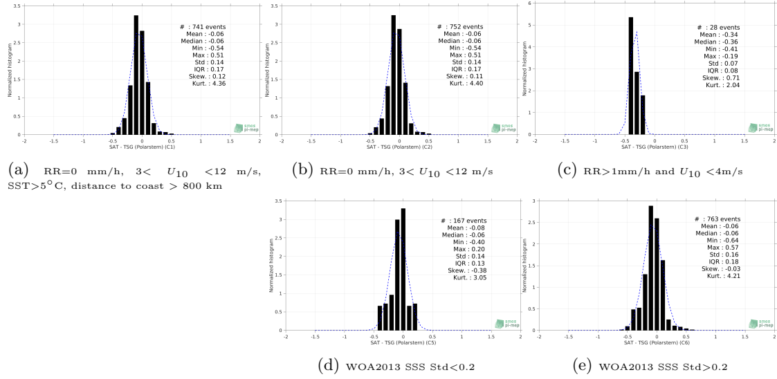
Figure 13: Normalized histogram of \Delta SSS (CCI L4 Merged-OI v2.31 - 7-day running (ESA) - TSG (Polarstern)) for 5 different subdatasets corresponding to: RR=0 mm/h, 3 < U_{10} < 12 m/s, SST>5°C, distance to coast > 800 km (a), RR=0 mm/h, 3 < U_{10} < 12 m/s (b), RR>1mm/h and U_{10} < 4 m/s (c), WOA2013 SSS Std<0.2 (d), WOA2013 SSS Std>0.2 (e).
