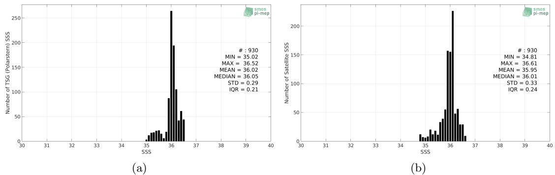
Figure 2: Histograms of SSS from TSG (Polarstern) (a) and CCI L4 Merged-OI v2.31 - 7-day running (ESA) (b) considering all match-up pairs per bins of 0.1 over the Amazon and Orinoco river plumes Pi-MEP region and for the full satellite product period.
