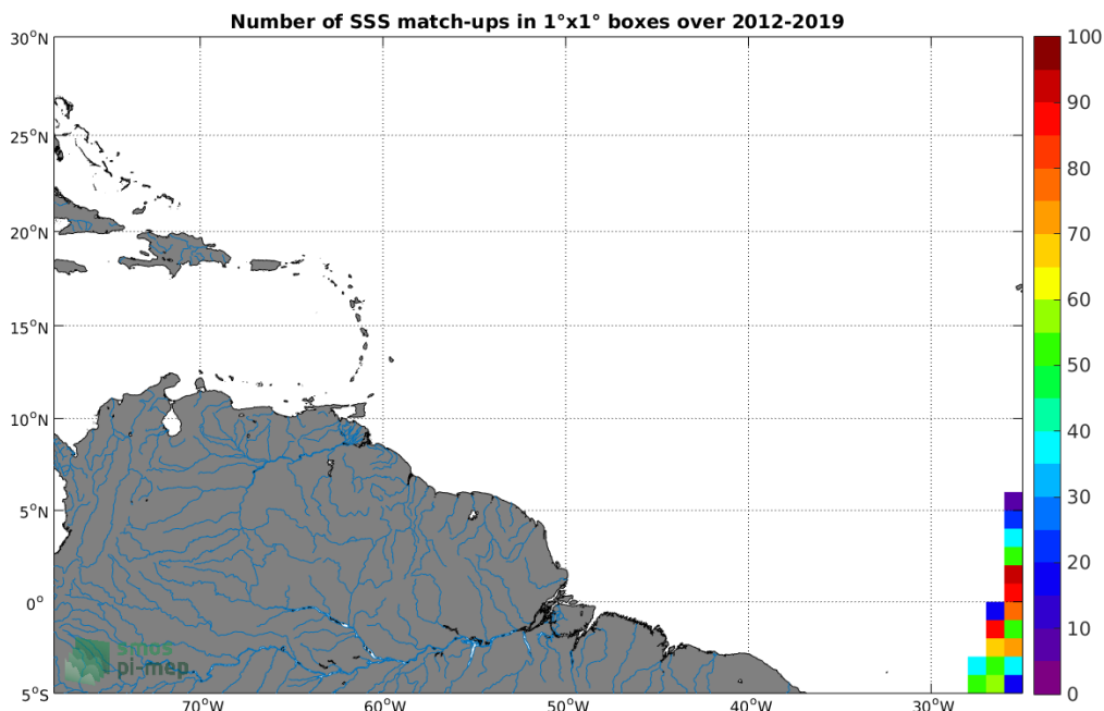
Figure 4: Number of SSS match-ups between TSG (Polarstern) SSS and the CCI L4 Merged-OI v2.31 - 7-day running (ESA) SSS product for the Amazon and Orinoco river plumes Pi-MEP region over 1°x1° boxes and for the full satellite product period.
