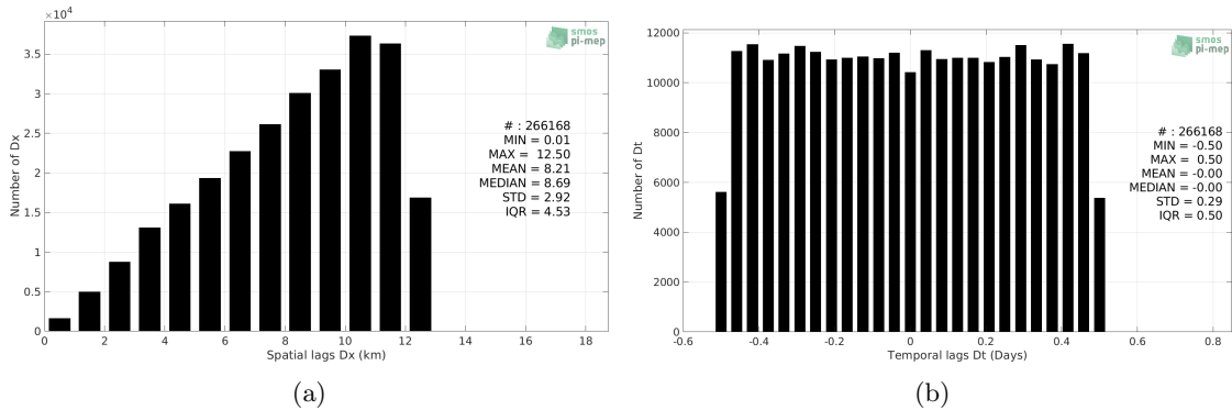
Figure 5: Histograms of the spatial (a) and temporal (b) lags between the location/time of the TSG (LEGOS-DM) measurement and the date of the corresponding CCI SSS L4 Merged-OI v2.31 - 7-day running (ESA) SSS pixel.
