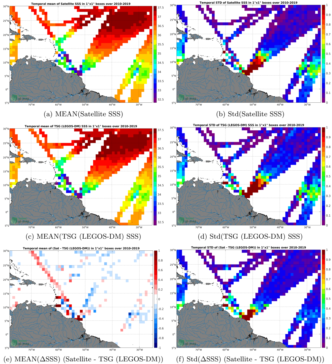
Figure 6: Temporal mean (left) and Std (right) of SSS from CCI SSS L4 Merged-OI v2.31 - 7-day running (ESA) (top), TSG (LEGOS-DM) (middle), and of \Delta SSS (Satellite - TSG (LEGOS-DM)). Only match-up pairs are used to generate these maps.
