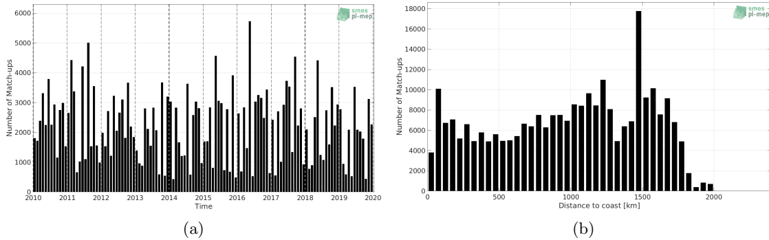
Figure 1: Number of match-ups between TSG (LEGOS-DM) and CCI SSS L4 Merged-OI v2.31 - 7-day running (ESA) SSS as a function of time (a) and as function of the distance to coast (b) over the Amazon and Orinoco river plumes Pi-MEP region and for the full satellite product period.
