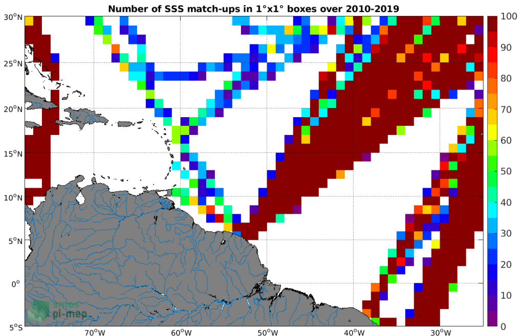
Figure 4: Number of SSS match-ups between TSG (LEGOS-DM) SSS and the CCI SSS L4 Merged-OI v2.31 - 7-day running (ESA) SSS product for the Amazon and Orinoco river plumes Pi-MEP region over 1^{\circ} \times 1^{\circ} boxes and for the full satellite product period.
