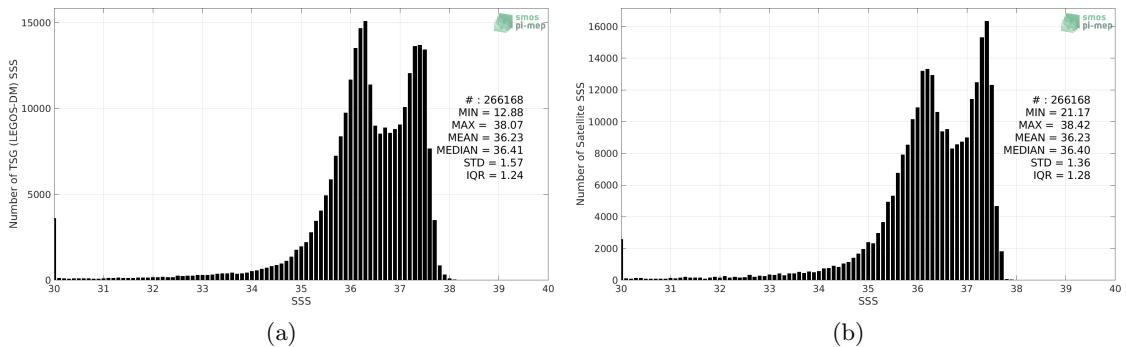
Figure 2: Histograms of SSS from TSG (LEGOS-DM) (a) and CCI SSS L4 Merged-OI v2.31 - 7-day running (ESA) (b) considering all match-up pairs per bins of 0.1 over the Amazon and Orinoco river plumes Pi-MEP region and for the full satellite product period.
