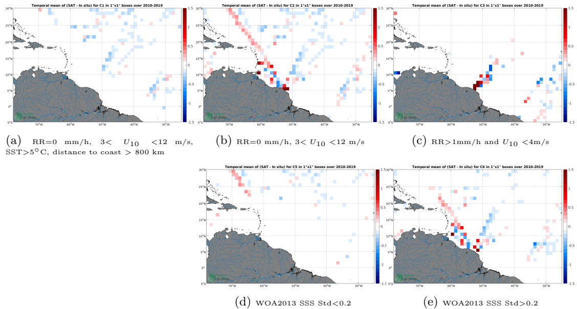
Figure 12: Temporal mean gridded over spatial boxes of size 1^{\circ}\times 1^{\circ} of \Delta\text{SSS} (CCI SSS L4 Merged-OI v2.31 - 7-day running (ESA) - TSG (LEGOS-DM)) for 5 different subdatasets corresponding to:RR=0 mm/h, 3 < U_{10} < 12 m/s, SST >5^{\circ}\text{C} , distance to coast > 800 km (a), RR=0 mm/h, 3 < U_{10} < 12 m/s (b), RR >1 mm/h and U_{10} < 4 m/s (c), WOA2013 SSS Std <0.2 (d), WOA2013 SSS Std >0.2 (e).
