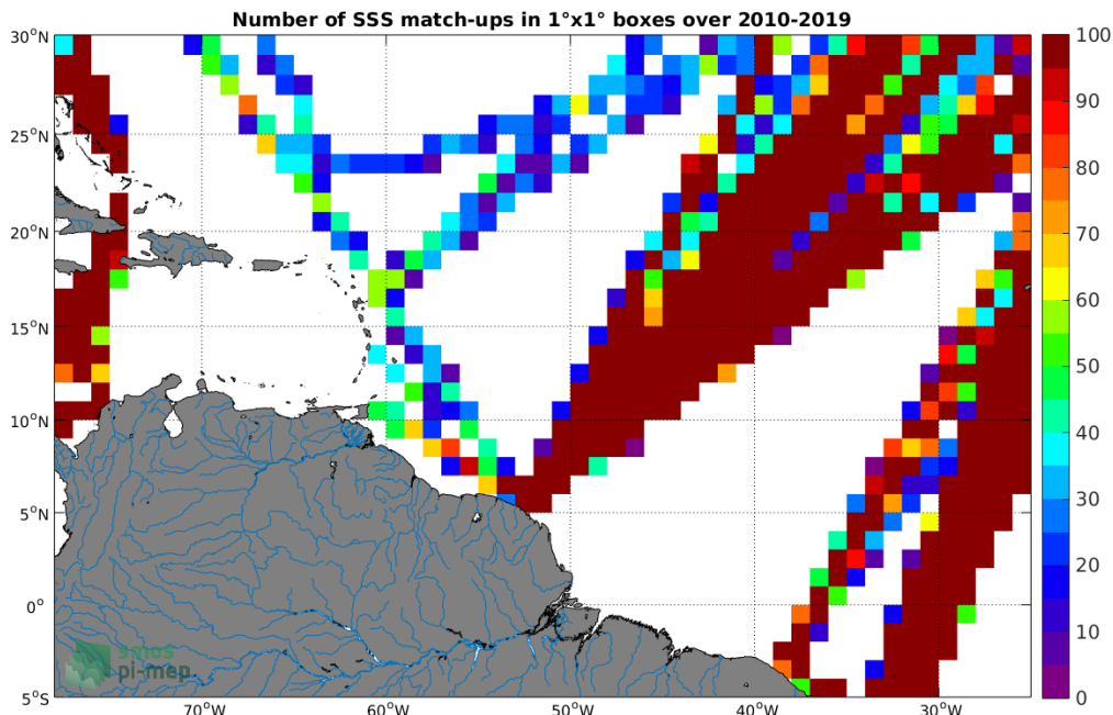
Figure 4: Number of SSS match-ups between TSG (LEGOS-DM) SSS and the CCI L4 Merged-OI v2.31 - 7-day running (ESA) SSS product for the Amazon and Orinoco river plumes Pi-MEP region over 1°x1° boxes and for the full satellite product period.
