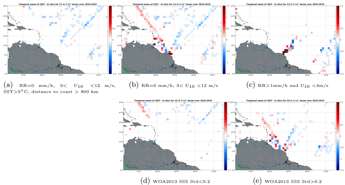
Figure 12: Temporal mean gridded over spatial boxes of size 1^\circ \times 1^\circ of \Delta SSS (CCI L4 Merged-OI v2.31 - 7-day running (ESA) - TSG (LEGOS-DM)) for 5 different subdatasets corresponding to:RR=0 mm/h, 3 < U_{10} < 12 m/s, SST >5^\circ C, distance to coast > 800 km (a), RR=0 mm/h, 3 < U_{10} < 12 m/s (b), RR >1 mm/h and U_{10} < 4 m/s (c), WOA2013 SSS Std <0.2 (d), WOA2013 SSS Std >0.2 (e).
