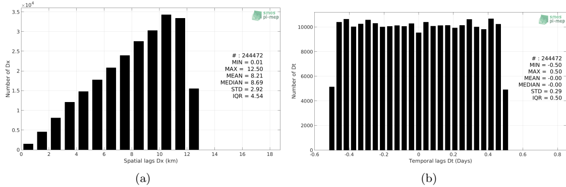
Figure 5: Histograms of the spatial (a) and temporal (b) lags between the time of the TSG (LEGOS-DM) measurements and the date of the corresponding CCI L4 Merged-OI v2.31 - 7-day running (ESA) SSS product.
