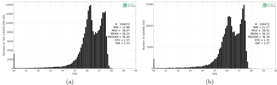
Figure 2: Histograms of SSS from TSG (LEGOS-DM) (a) and CCI L4 Merged-OI v2.31 - 7-day running (ESA) (b) considering all match-up pairs per bins of 0.1 over the Amazon and Orinoco river plumes Pi-MEP region and for the full satellite product period.
