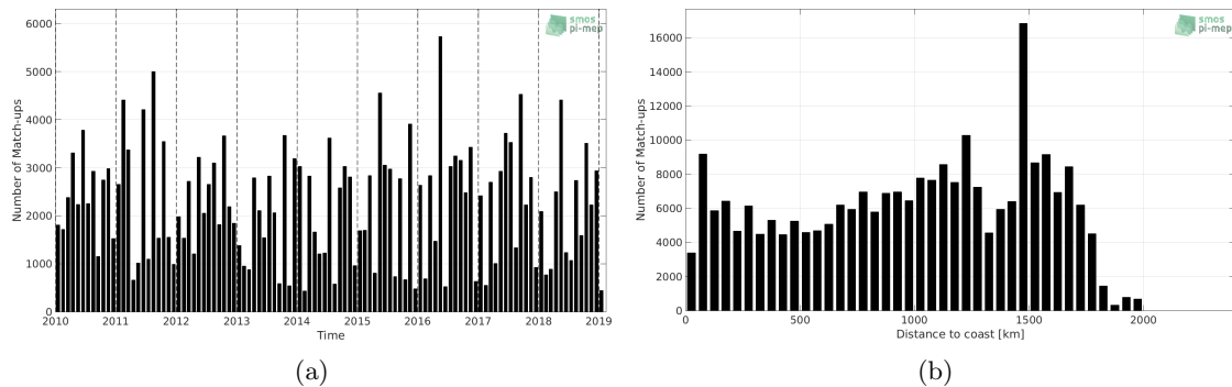
Figure 1: Number of match-ups between TSG (LEGOS-DM) and CCI L4 Merged-OI v2.31 - 7-day running (ESA) SSS as a function of time (a) and as function of the distance to coast (b) over the Amazon and Orinoco river plumes Pi-MEP region and for the full satellite product period.
