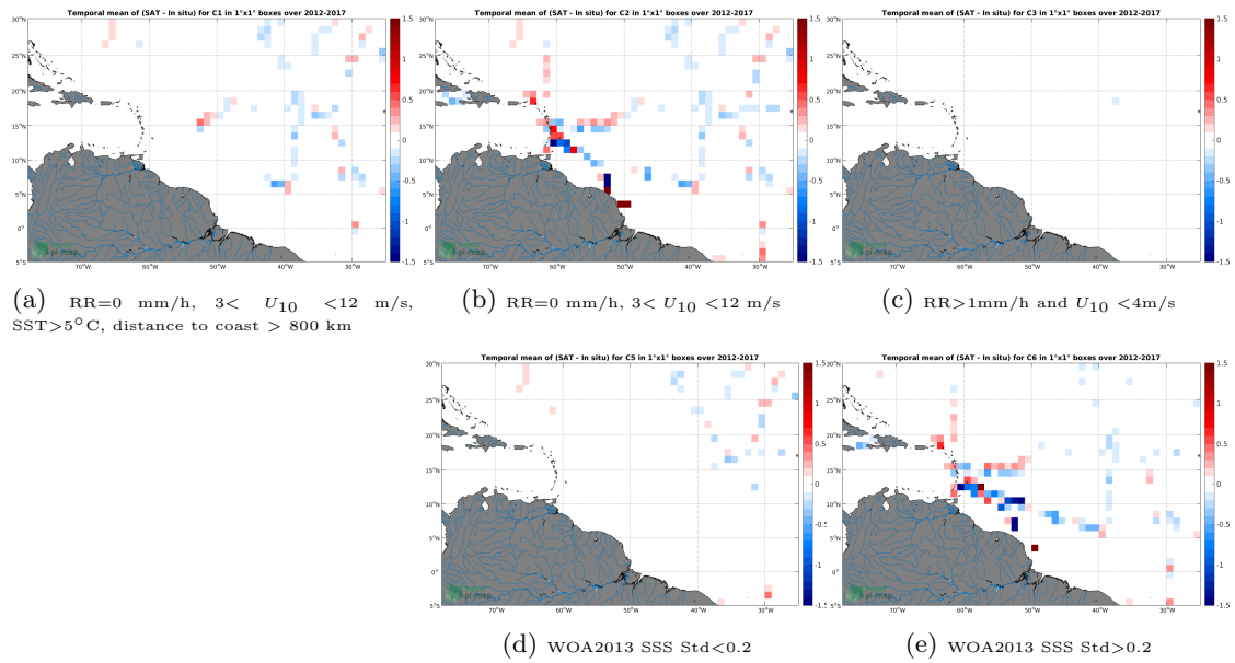
Figure 12: Temporal mean gridded over spatial boxes of size 1^{\circ}\times 1^{\circ} of \Delta SSS (CCI SSS L4 Merged-OI v2.31 - 7-day running (ESA) - TSG (GOSUD-Sailing-ship)) for 5 different subdatasets corresponding to:RR=0 mm/h, 3 < U_{10} < 12 m/s, SST >5^{\circ}\text{C} , distance to coast > 800 km (a), RR=0 mm/h, 3 < U_{10} < 12 m/s (b), RR >1 mm/h and U_{10} < 4 m/s (c), WOA2013 SSS Std <0.2 (d), WOA2013 SSS Std >0.2 (e).
