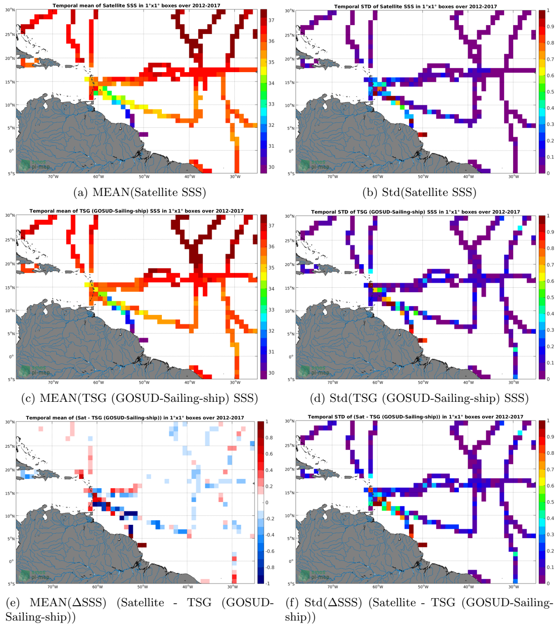
Figure 6: Temporal mean (left) and Std (right) of SSS from CCI SSS L4 Merged-OI v2.31 - 7-day running (ESA) (top), TSG (GOSUD-Sailing-ship) (middle), and of \Delta SSS (Satellite - TSG (GOSUD-Sailing-ship)). Only match-up pairs are used to generate these maps.
