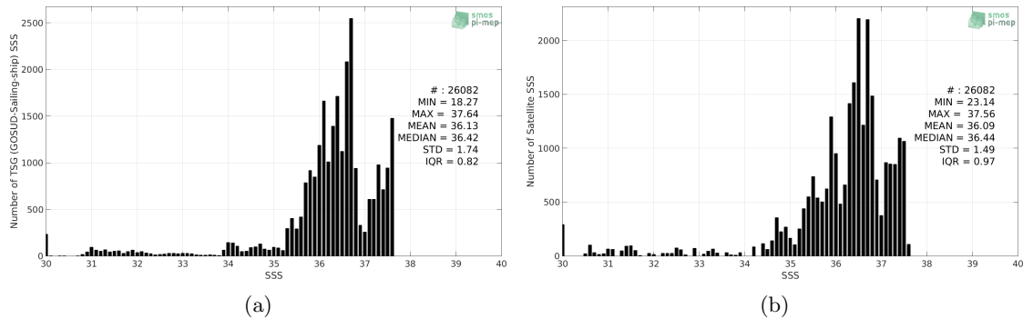
Figure 2: Histograms of SSS from TSG (GOSUD-Sailing-ship) (a) and CCI SSS L4 Merged-OI v2.31 - 7-day running (ESA) (b) considering all match-up pairs per bins of 0.1 over the Amazon and Orinoco river plumes Pi-MEP region and for the full satellite product period.
