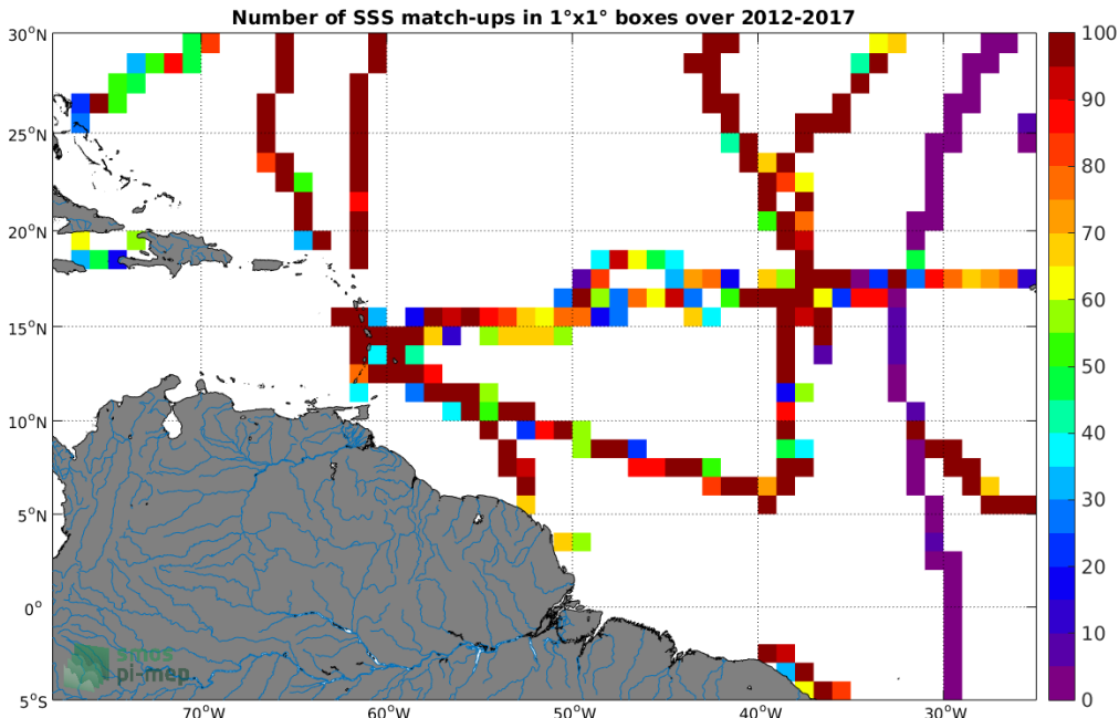
Figure 4: Number of SSS match-ups between TSG (GOSUD-Sailing-ship) SSS and the CCI SSS L4 Merged-OI v2.31 - 7-day running (ESA) SSS product for the Amazon and Orinoco river plumes Pi-MEP region over 1^\circ \times 1^\circ boxes and for the full satellite product period.
